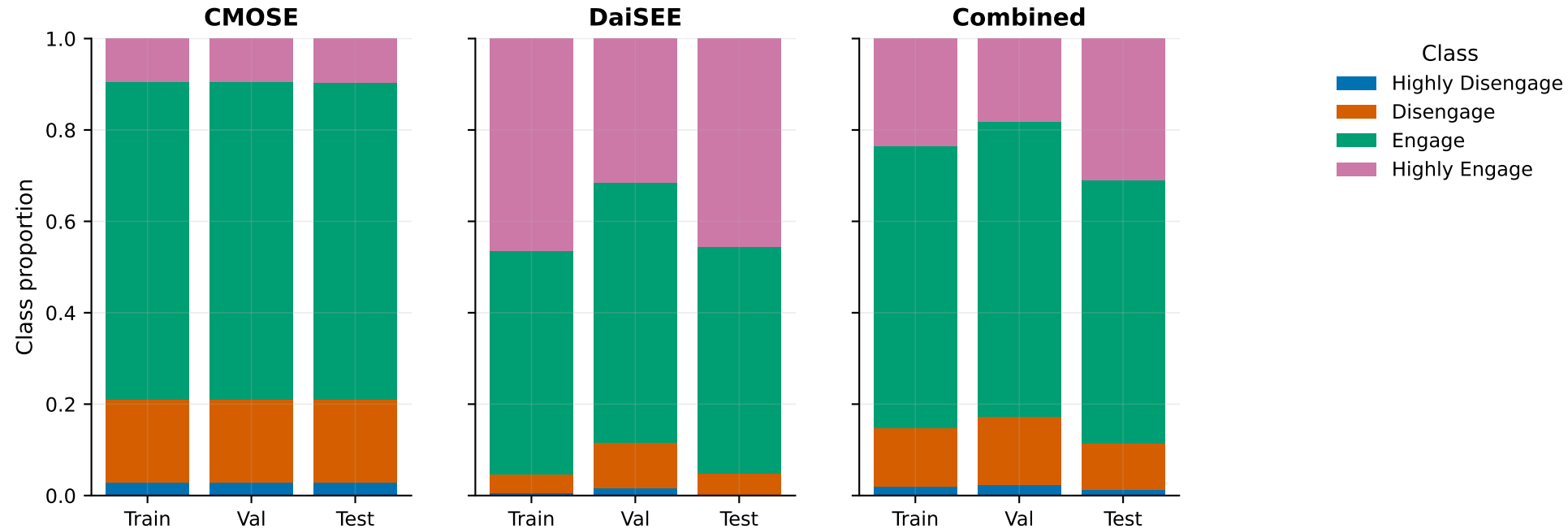
Class distribution per train / val / test split
