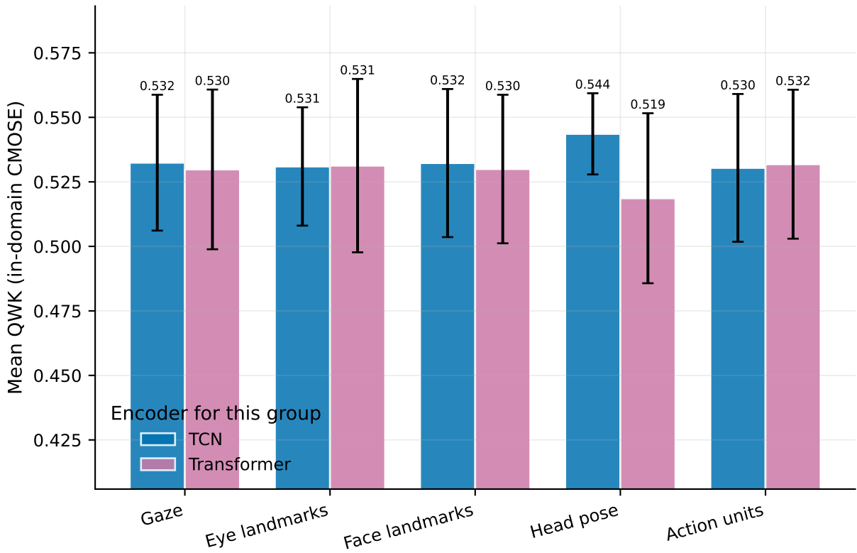
Per-group marginal effect of encoder choice (TCN vs Transformer)
