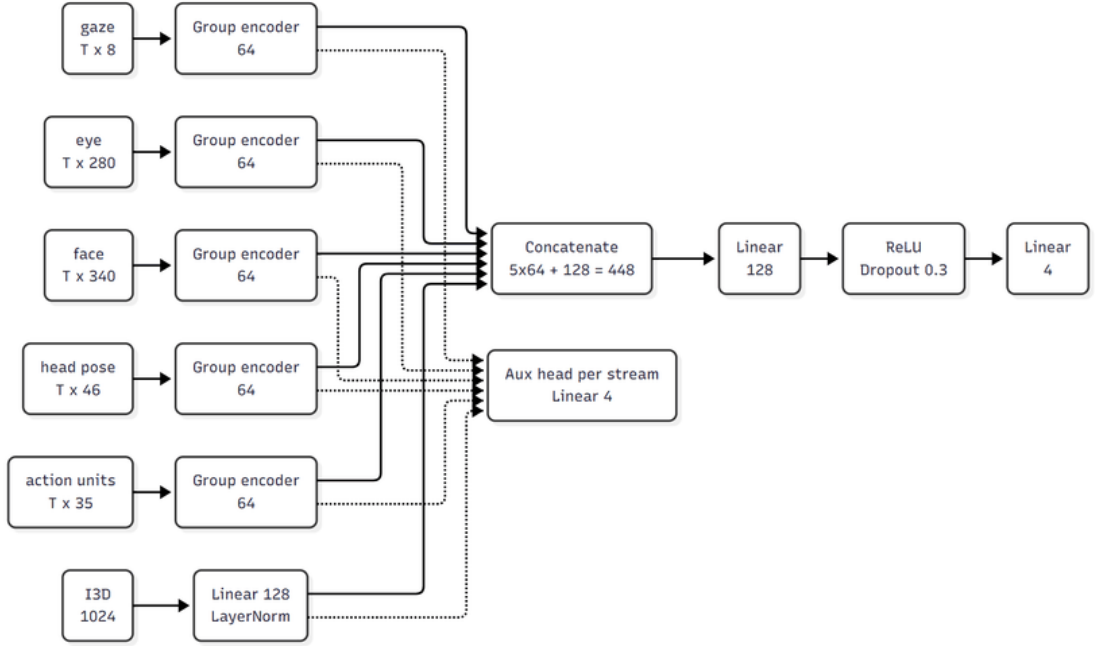
Figure 3.3: Semantic-group hybrid architecture. Each OpenFace group is encoded independently into a 64-d embedding (group encoders are chosen per group from TCN / Transformer (T) / LSTM); the I3D clip vector is encoded by an MLP into a 128-d embedding. The six embeddings are concatenated (448-d) and classified by a shared MLP; each stream also feeds an auxiliary head. The OpenFace-only variant drops the I3D row and fuses a 320-d vector.
