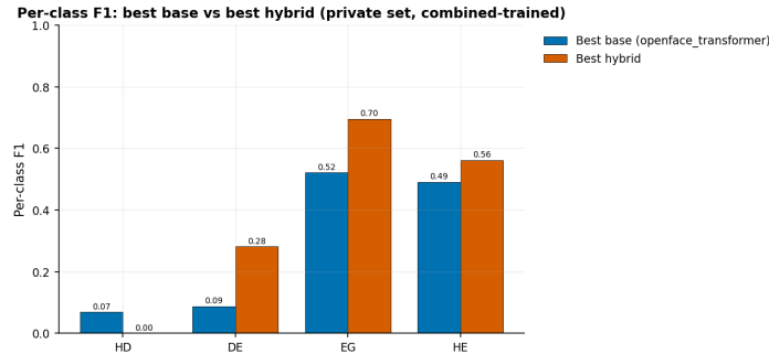
Figure 5.5: Per-class F1 on the private set: combined-trained best base model versus best hybrid. The hybrid’s out-of-domain gain concentrates on the engaged region and the middle Disengage class, while Highly-Disengage collapses to zero.
