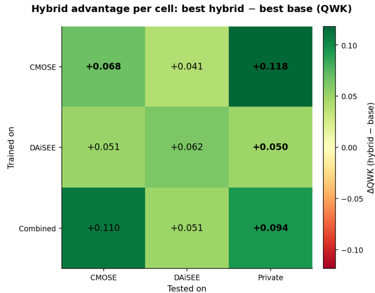
Figure 5.3: Cell-by-cell hybrid advantage: best-hybrid minus best-base QWK over the 3 \times 3 train \times test matrix (Figure 5.2 minus Figure 4.5). Every cell is positive — the hybrid wins the whole matrix — and the gain is largest on the unseen, self-collected Private column. The in-domain CMOSE cell and the Private column (bold) are the two comparisons read in Sections 5.5 and 5.6.2.
