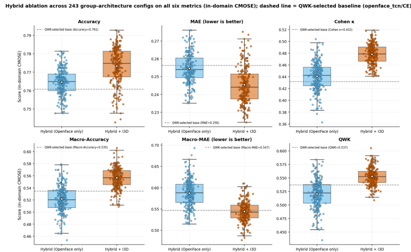
Figure 5.1: Hybrid ablation across all 243 per-group encoder configurations, with and without I3D, on all six metrics (in-domain CMOSE). The dashed line in every panel is the same model — the single QWK-selected baseline (OpenFace TCN, cross-entropy) — read on that panel’s metric, not a per-metric champion.
