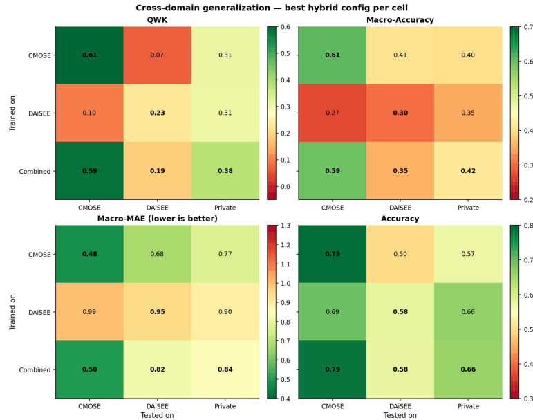
Figure 5.2: Cross-domain generalisation, best hybrid per cell (selected by QWK), on QWK — the selection metric — and the balanced secondary metrics macro-accuracy and macro-MAE (lower is better), plus raw accuracy, which again stays high in the off-diagonal cells where the chance-corrected metrics collapse.
