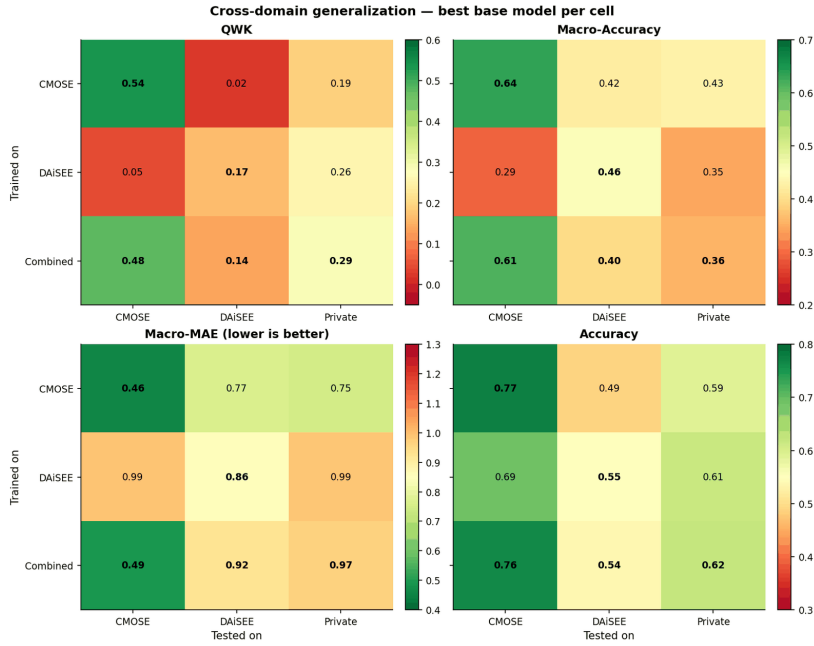
Figure 4.5: Cross-domain generalisation, best base model per cell (selected by QWK), on QWK — the selection metric — and the balanced secondary metrics macro-accuracy and macro-MAE (lower is better), plus raw accuracy, the deceptive foil: accuracy stays high in exactly the off-diagonal cells where every chance-corrected metric collapses.
