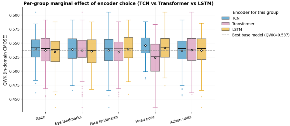
Figure 5.2: Per-group marginal effect of the encoder choice on in-domain QWK.
