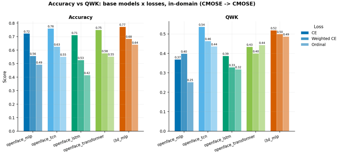
Figure 4.1: Accuracy versus QWK for the five base models under the three losses, in-domain on CMOSE: accuracy ranks the I3D MLP first while QWK ranks the OpenFace TCN first.
