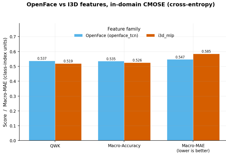
Figure 4.5: Best OpenFace encoder (the TCN) versus the I3D MLP on the three primary metrics, in-domain on CMOSE under cross-entropy: OpenFace wins all three.
