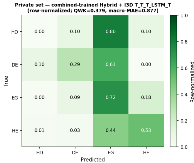
Figure 5.8: Private-set confusion, combined-trained I3D hybrid T_T_T_LSTM_T (QWK 0.379, macro-MAE 0.877), row-normalised.
