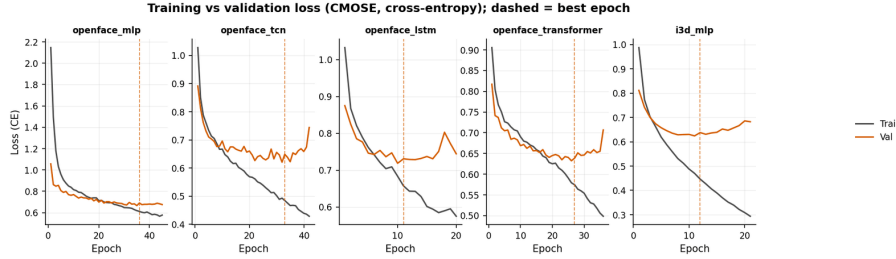
Figure 4.4: Representative training/validation loss curves (CMOSE, cross-entropy).
