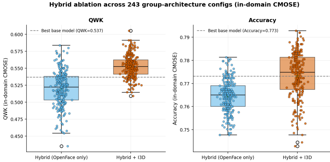
Figure 5.1: Hybrid ablation across all 243 per-group encoder configurations, with and without I3D, on QWK (higher is better) and accuracy, against the best baseline.
