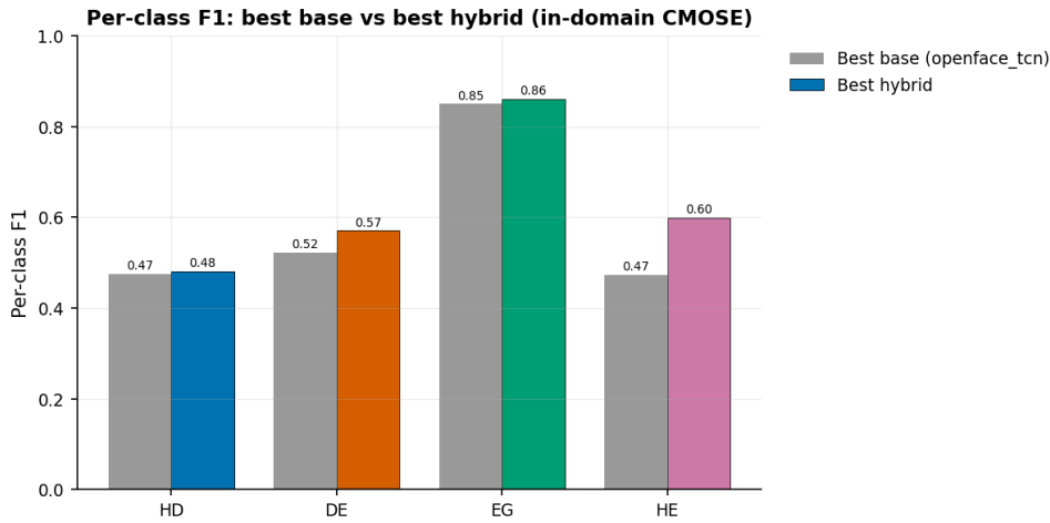
Figure 5.5: Per-class F1: best base versus best hybrid.
