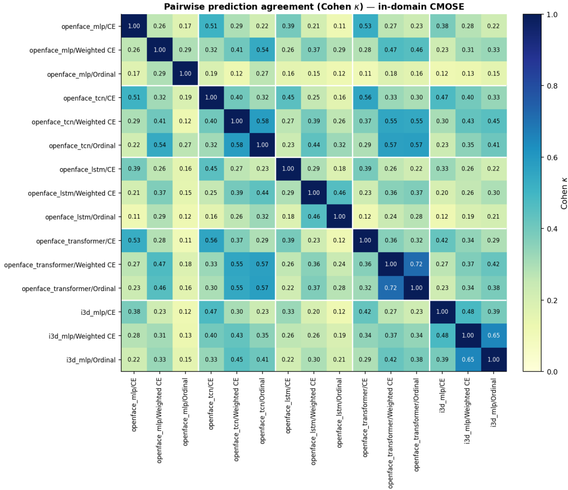
Figure 4.4: Pairwise prediction agreement (Cohen’s \kappa ) between all fifteen baseline configurations on the in-domain CMOSE test set, in model-major blocks.
