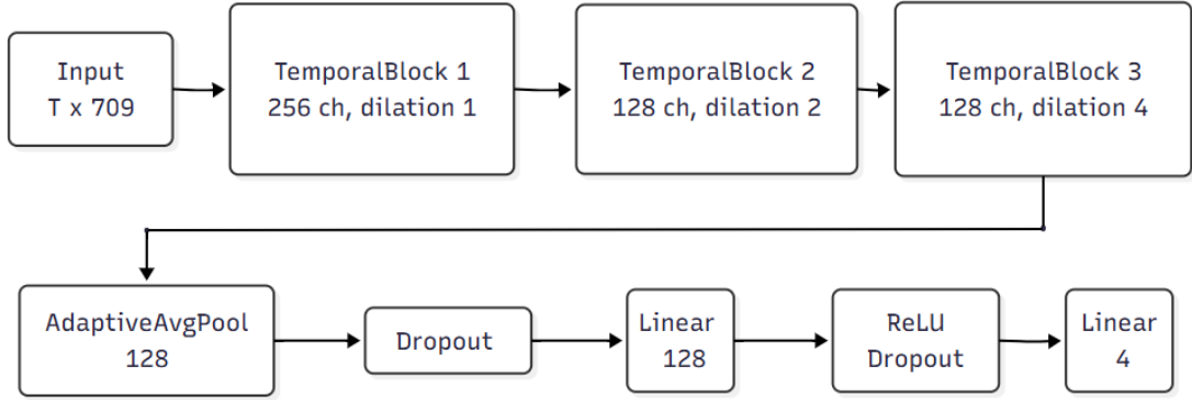
(b) openface_tcn.
