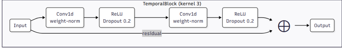
Figure 2.1: Residual TemporalBlock
