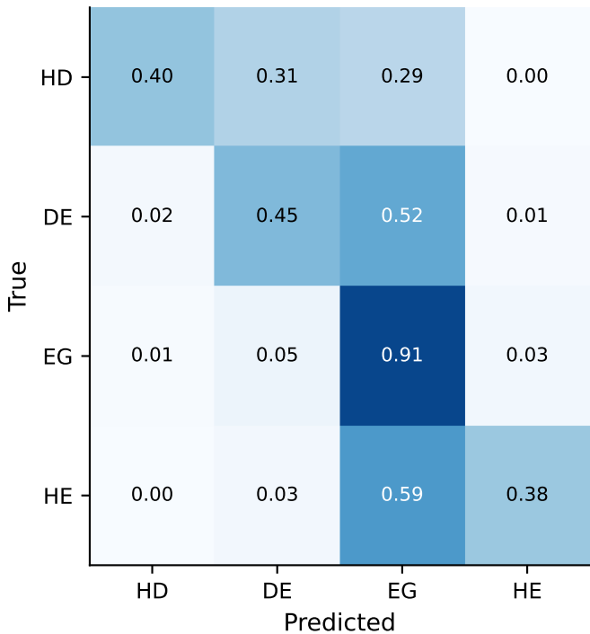
Best base: openface_tcn / ce QWK=0.537
