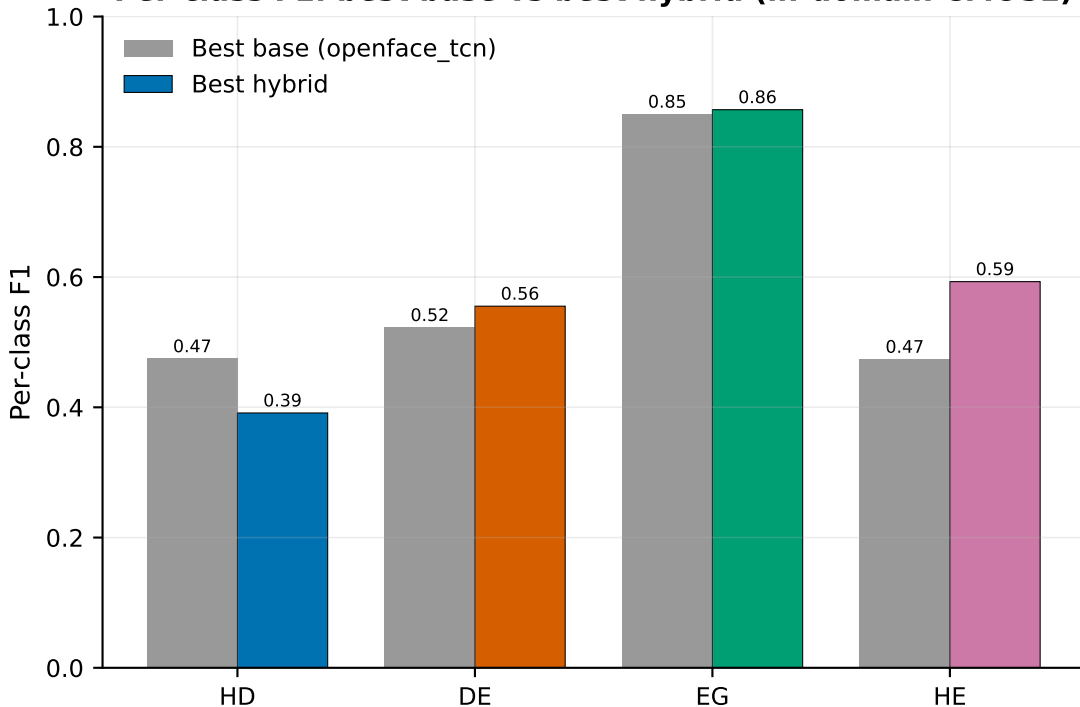
Per-class F1: best base vs best hybrid (in-domain CMOSE)
