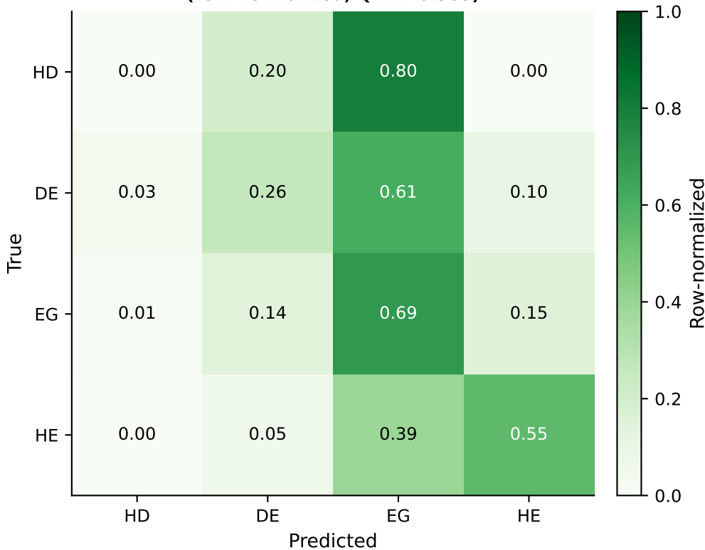
Private set — combined-trained Hybrid + I3D T_T_T_T_TCN (row-normalized; QWK=0.365)
