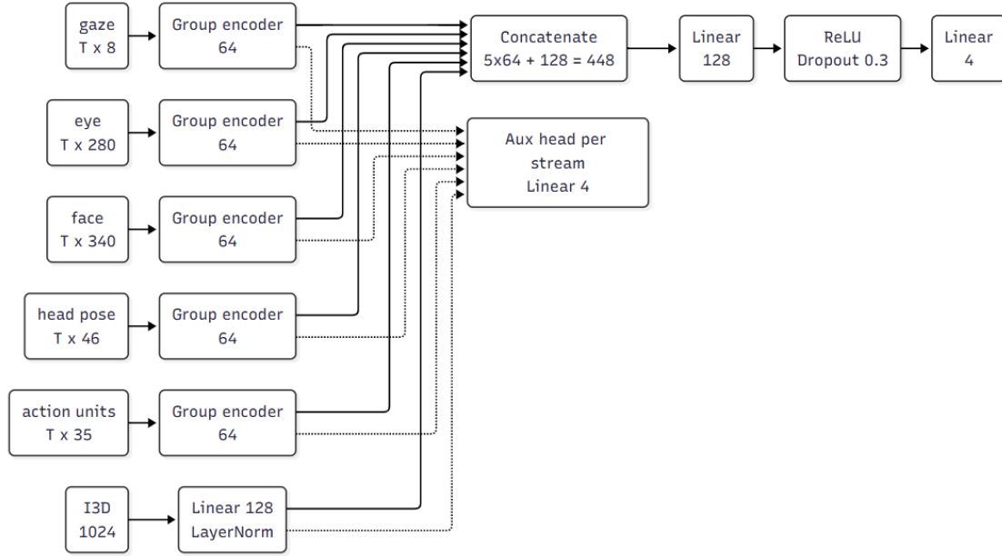
Figure 3.5: Proposed hybrid model architecture (I3D stream enabled; the I3D-stream-disabled variant drops the I3D row).
