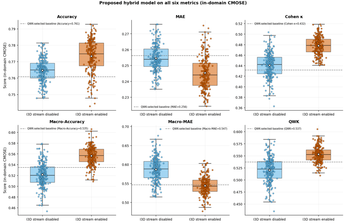
Figure 4.1: Ablation of the proposed hybrid model across all 243 per-group encoder configurations, with the I3D stream enabled and disabled, on all six metrics (in-domain CMOSE). The dashed line is the QWK-selected baseline (OpenFace TCN, cross-entropy).
