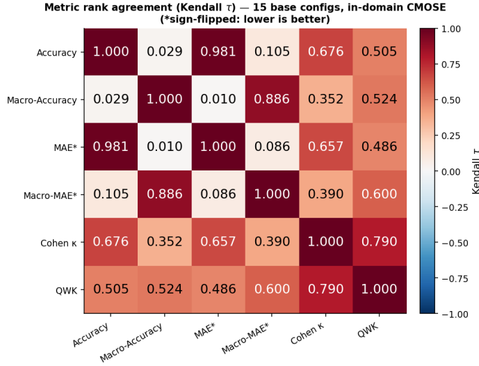
Figure A.1: Rank agreement (Kendall \tau ) between the six metrics over the fifteen baseline configurations, in-domain on CMOSE (MAE metrics sign-flipped so positive \tau means agreement).
