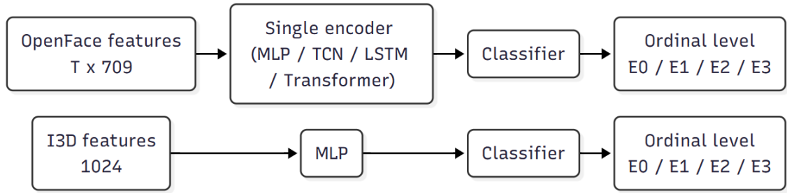
(a) Single-encoder baselines.
