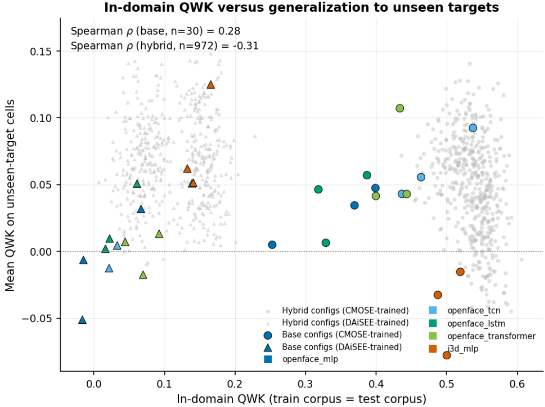
Figure 5.6: In-domain QWK versus mean unseen-target QWK with the hybrid ablation population overlaid on the baseline configurations. Within the hybrid family the correlation is negative ( \rho = -0.31 ): more in-domain fit means more dataset fit. The hybrid cloud lies above the baselines throughout: the architecture improves transfer at every level of in-domain performance.
