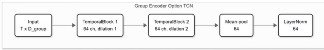
(a) TCN group encoder.
