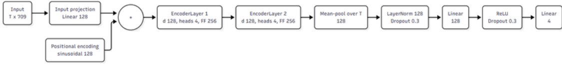
(d) openface_transformer : a Transformer encoder over the 709-d sequence, mean-pooled and classified.
