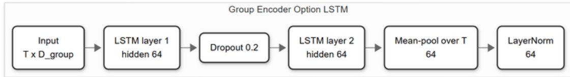
(c) LSTM group encoder.
