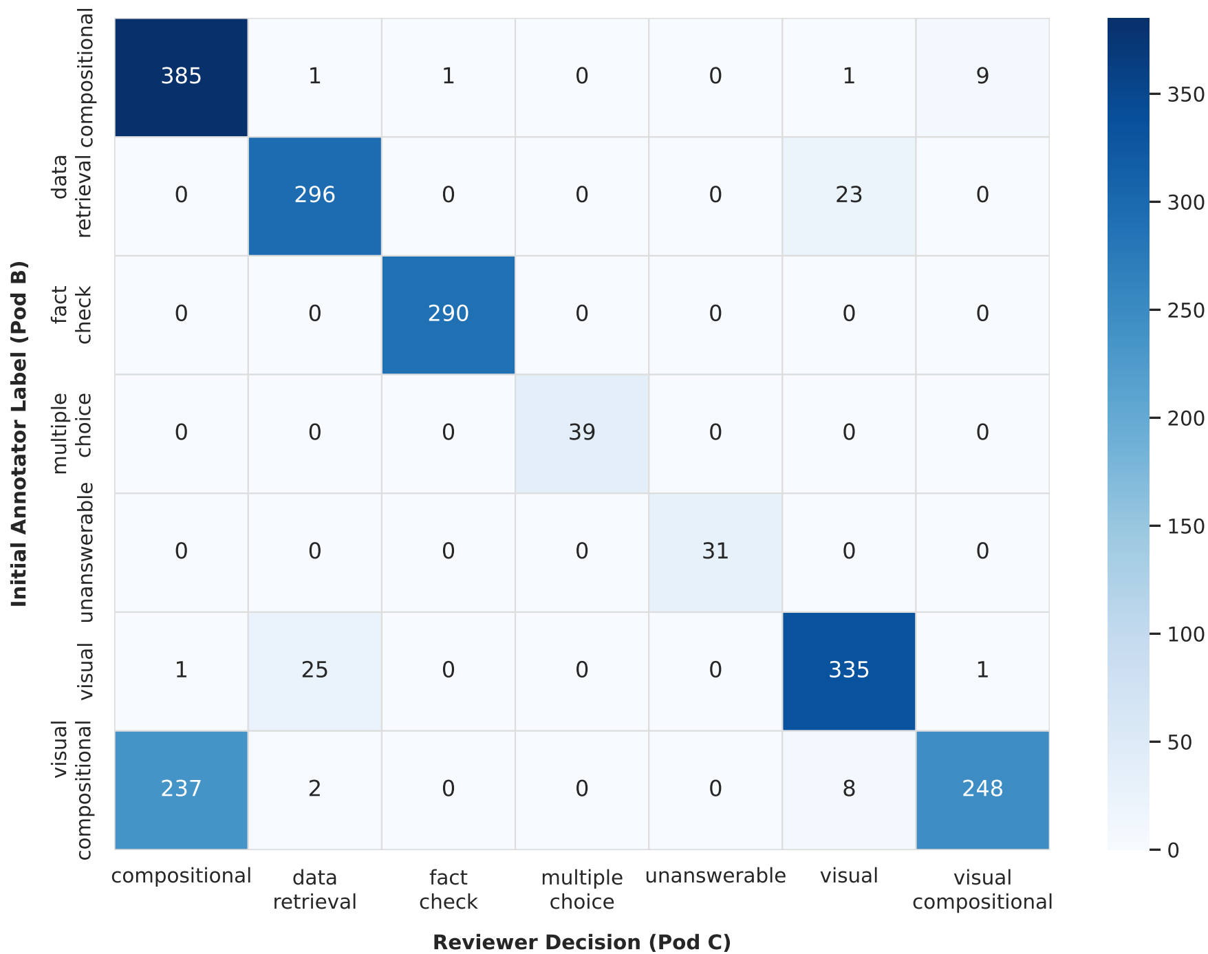
ViChartQA Inter-Annotator Agreement: Question Type Confusion Matrix (N = 1933, Observed Agreement = 84.0%, Cohen's \kappa = 0.8034)
