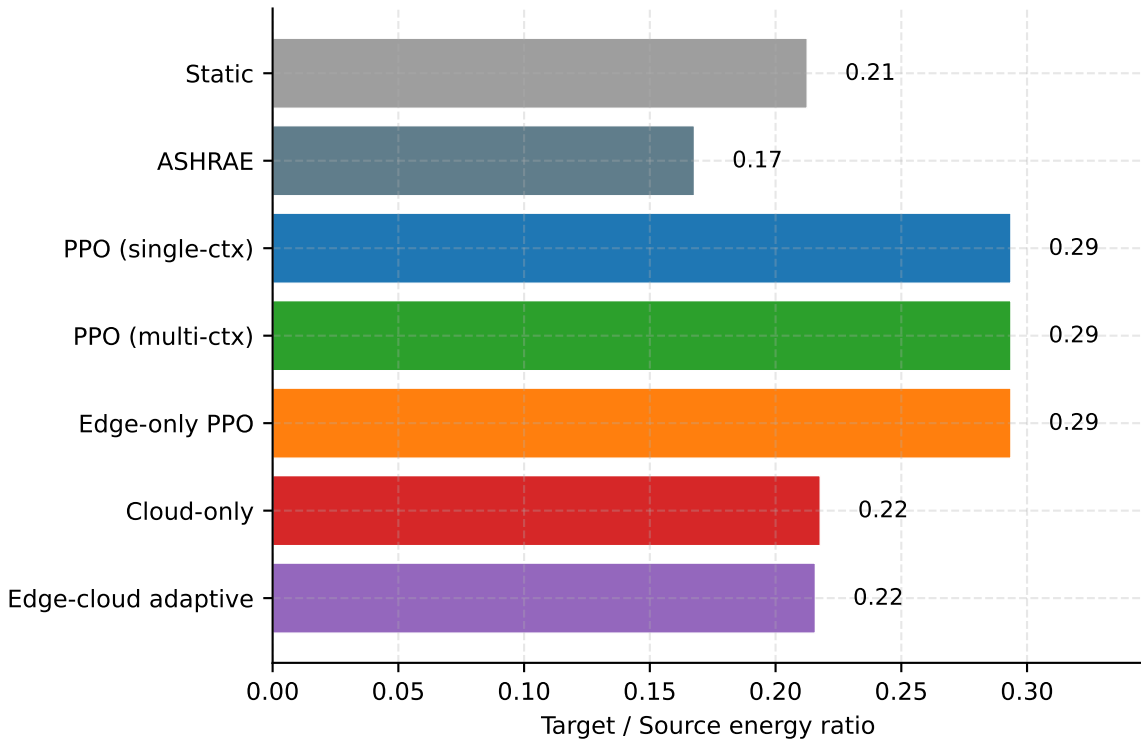
Transfer efficiency on target cities (DaNang, Hanoi)
