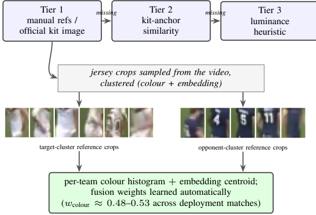
Fig. 2. Zero-manual-setup team-reference bootstrap (C2). A three-tier cascade selects which cluster of jersey crops is the target team; the chosen clusters become per-team references (colour histogram + vision-embedding centroid) with fusion weights learned automatically. Crops shown are an illustrative reconstruction on one daylight fixture using the same detect-crop-cluster procedure; they are torso-only and deliberately pixelated, since the deployed system stores only the resulting feature centroids, never images.
