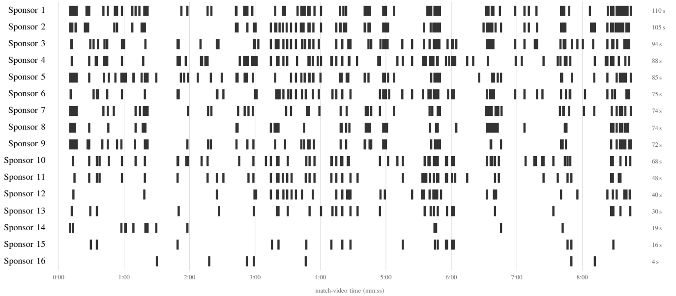
Fig. 3. Per-sponsor exposure timeline produced by the deployed pipeline for one club-captured highlight video (8.9 min, black-kit fixture, 2 fps analytics pass, team attribution enabled; this match’s attribution overlay was visually audited and assigns target/opponent correctly, §V-D). Each bar marks an interval in which the sponsor was detected on the target team’s kit after attribution; sponsors are sorted by total on-screen time (right column) and numbered rather than named, since sponsor names would identify the club whose identity we withhold. Very short intervals are widened to a minimum drawable width for legibility; totals are computed from the underlying segments, not from the drawing.
