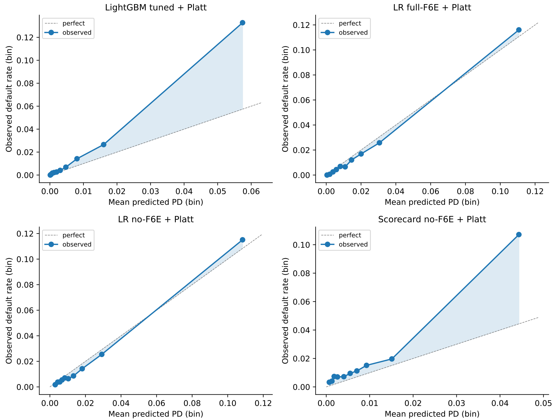
Figure 6 — Calibration reliability diagrams (10 deciles, OOT)
