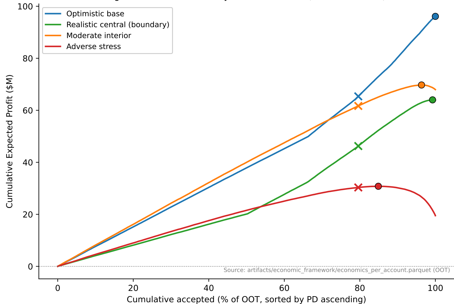
Figure 1 — Profit curves by anchor scenario (OOT, n=64,027)
