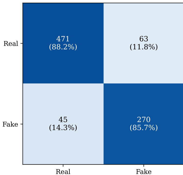
BiLSTM
