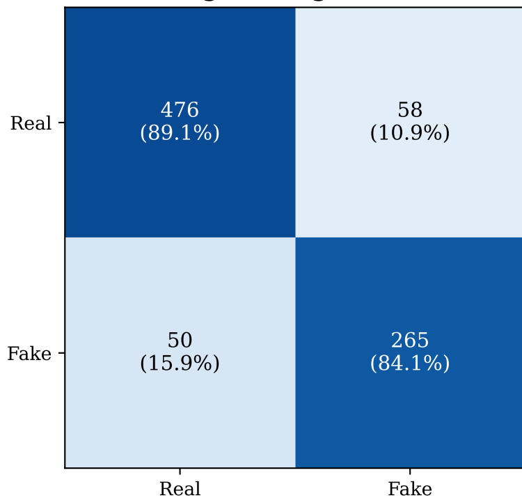
Logistic Regression
