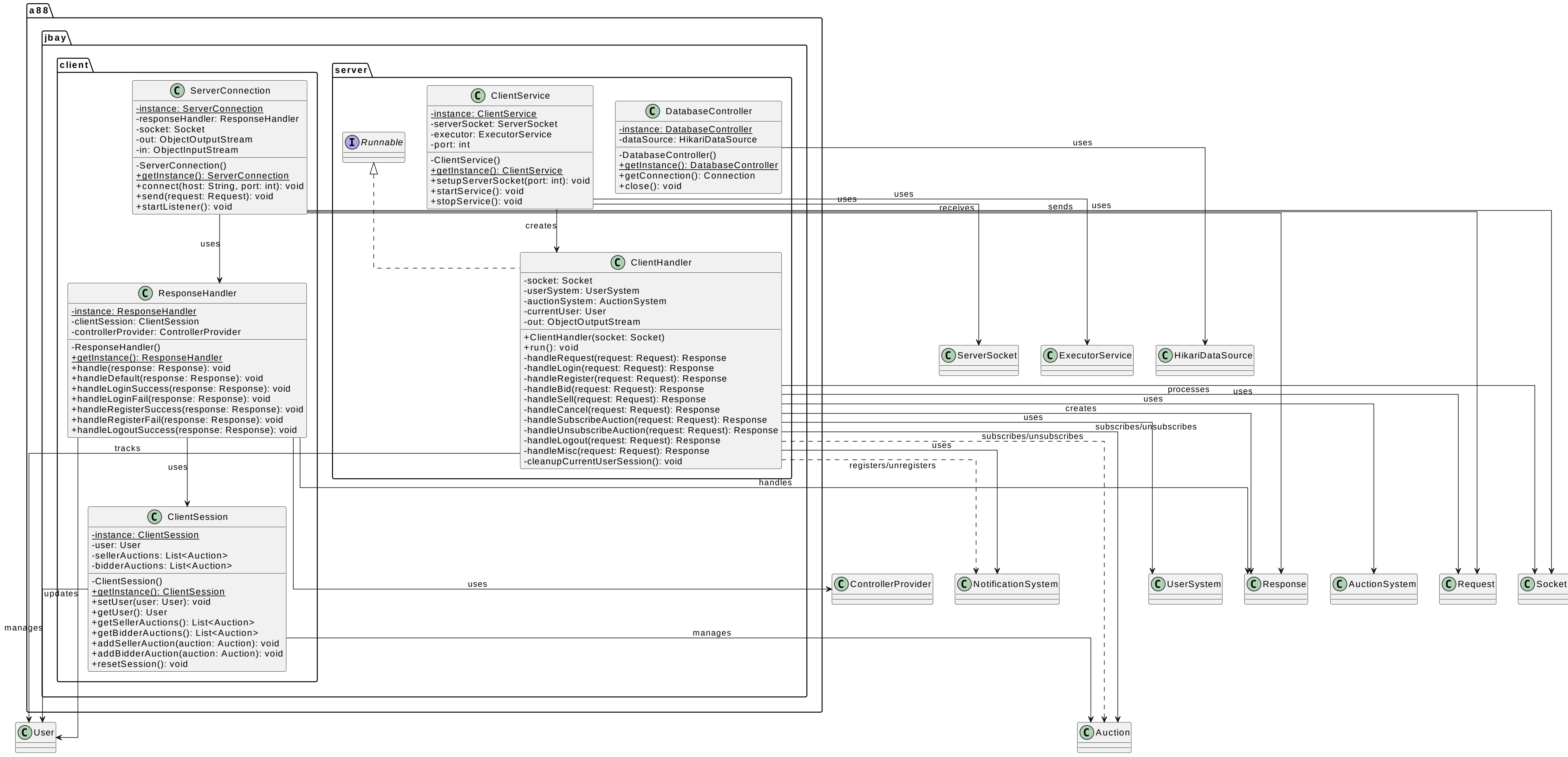
UML Diagram - a88.jbay.client and a88.jbay.server Packages
