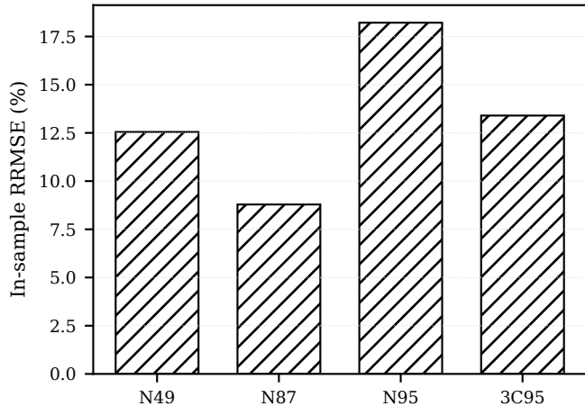
(a) Isothermal core-loss fits
