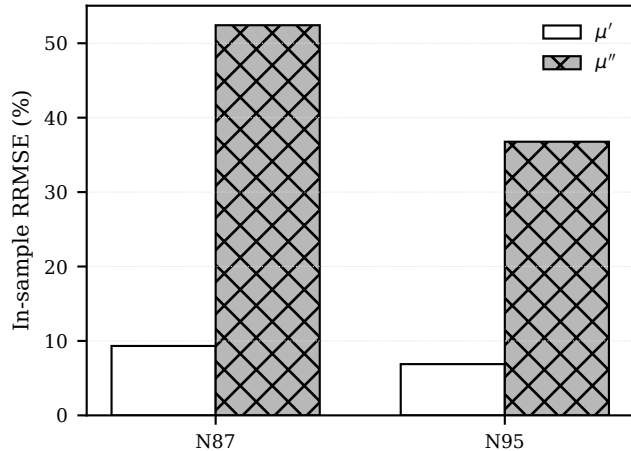
(b) Accepted permeability fits
