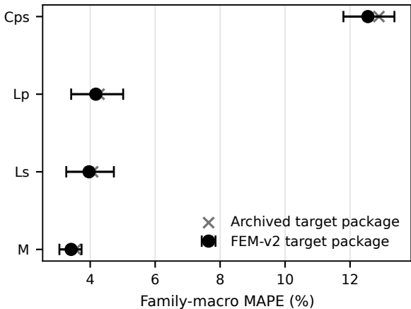
Family-held-out accuracy by target package
