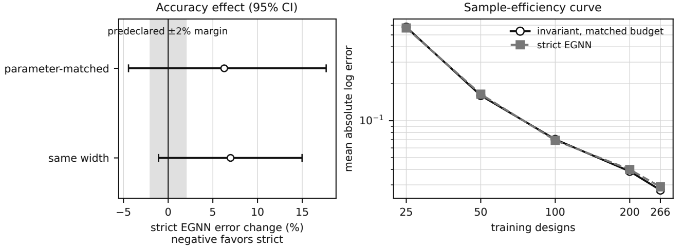
Fig. 3. Strict-coordinate-update ablation. Left: relative primary-error effects with paired hierarchical-bootstrap 95% intervals; the shaded band is the predeclared practical-equivalence margin. Right: five-seed mean learning curves on one fixed split. Exact encoded-graph symmetry is verified, but its accuracy and sample-efficiency effects are unresolved in the parameter-matched comparison.
