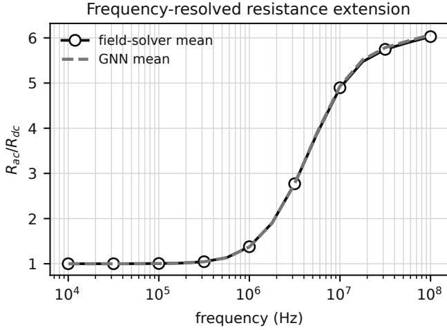
Fig. 6. Mean held-out R_{ac}/R_{dc}(f) curve for the separate frequency-resolved task. The 17-output model attains 0.37% median curve error over 27 test boards.
