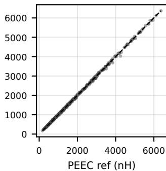
M R^2=0.9995
