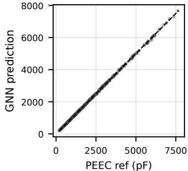
C_{ps} R^2=0.9998
