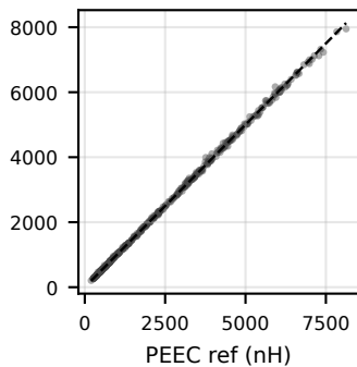
L_p R^2=0.9995
