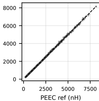
L_s R^2=0.9995
