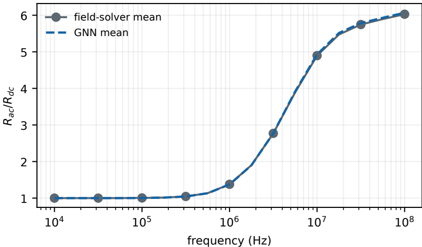
Frequency-resolved resistance extension
