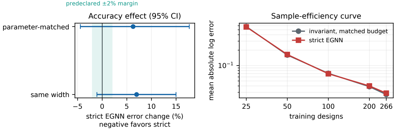
Fig. 3. Strict-coordinate-update ablation. Left: relative primary-error effects with paired hierarchical-bootstrap 95% intervals; the shaded band is the predeclared practical-equivalence margin. Right: five-seed mean learning curves on one fixed split. Exact encoded-graph symmetry is verified, but its accuracy and sample-efficiency effects are unresolved in the parameter-matched comparison.
