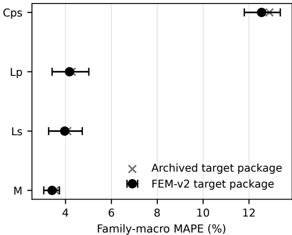
Version-scoped family-held-out accuracy
