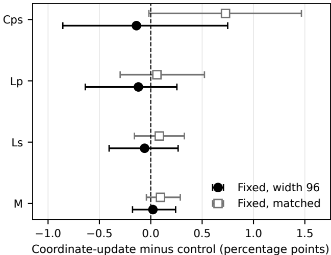
(a) Paired descriptive sensitivity intervals
