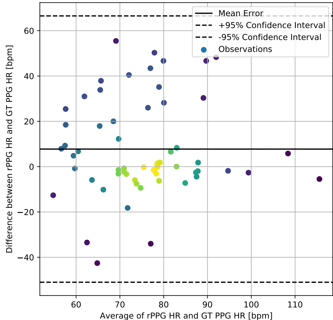
UBFC-rPPG_TSCAN_Custom_FFT_BlandAltman_DifferencePlot
