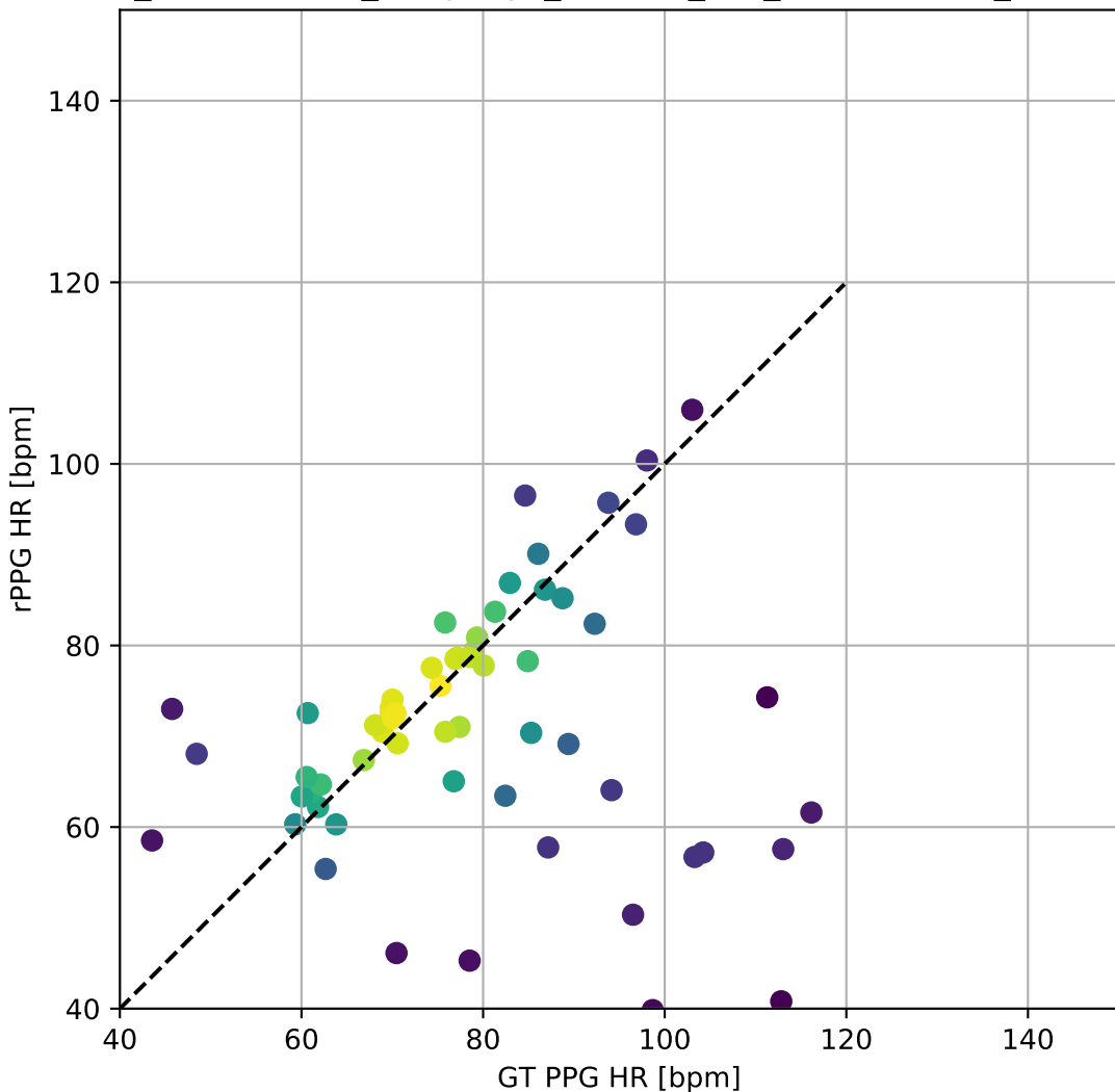
BP4D_PseudoLabel_DeepPhys_Custom_FFT_BlandAltman_ScatterPlot
