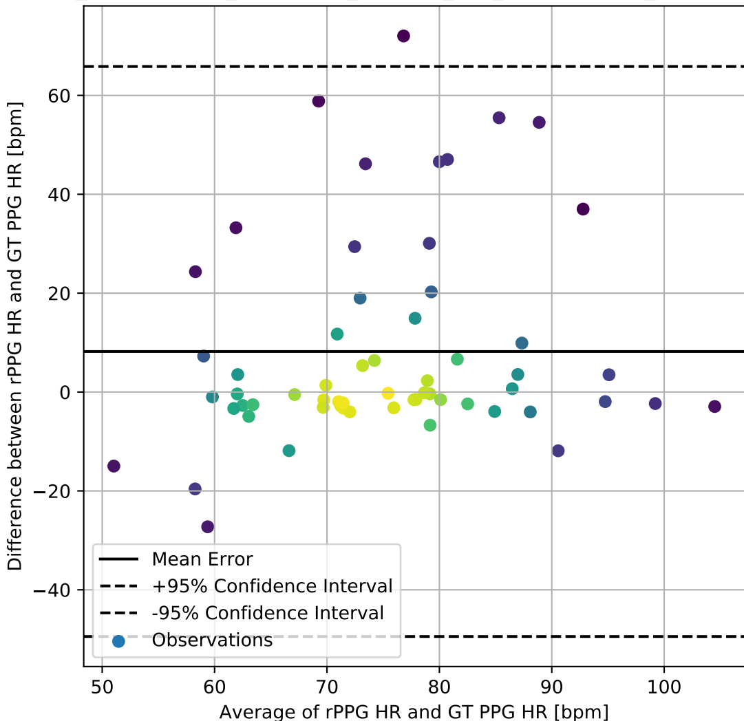
BP4D_PseudoLabel_DeepPhys_Custom_FFT_BlandAltman_DifferencePlot
