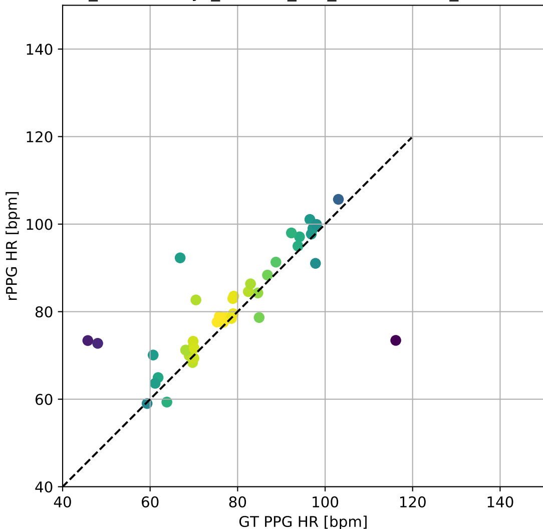
iBVP_EfficientPhys_Custom_FFT_BlandAltman_ScatterPlot
