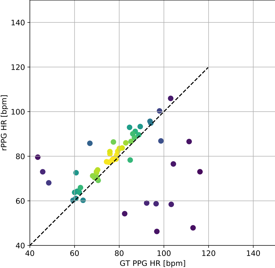
BP4D_PseudoLabel_EfficientPhys_Custom_FFT_BlandAltman_ScatterPlot
