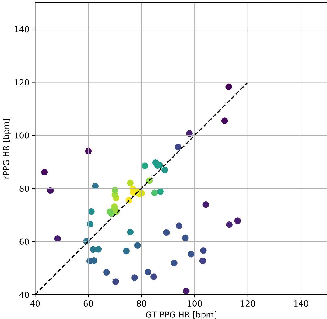
UBFC-rPPG_TSCAN_Custom_FFT_BlandAltman_ScatterPlot
