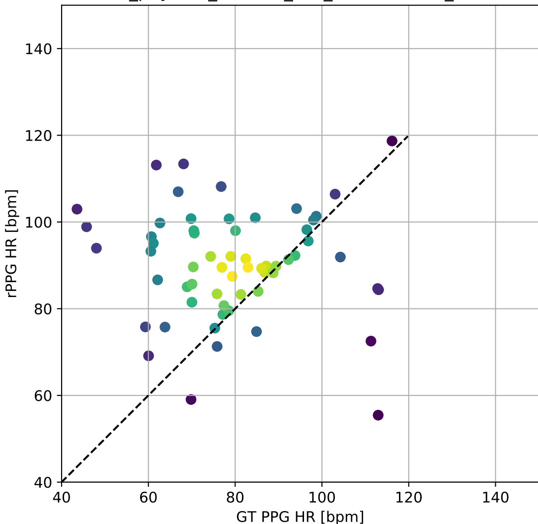
MA-UBFC_physnet_Custom_FFT_BlandAltman_ScatterPlot
