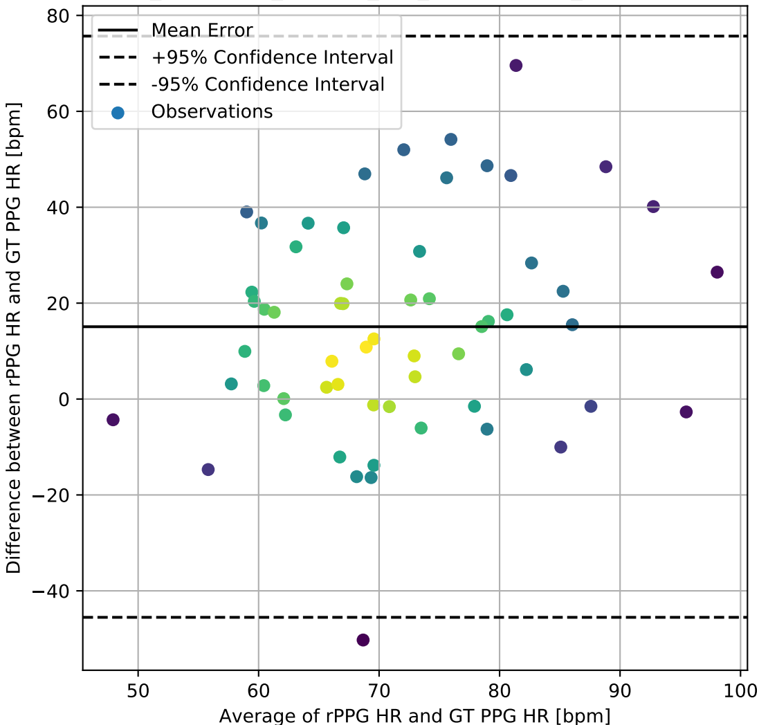
PURE_DeepPhys_Custom_FFT_BlandAltman_DifferencePlot
