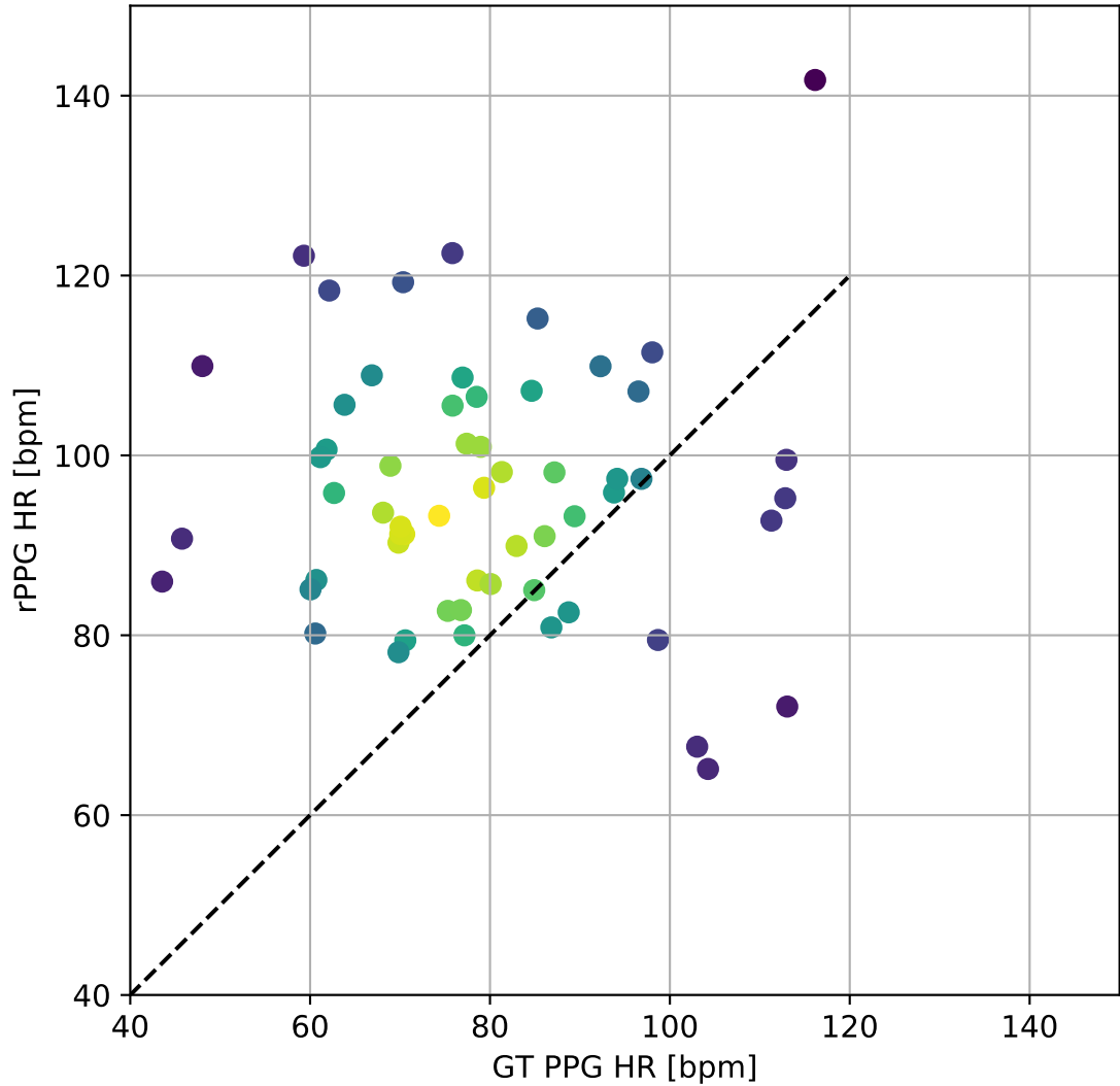
SCAMPS_PhysNet_DiffNormalized_Custom_FFT_BlandAltman_ScatterPlot
