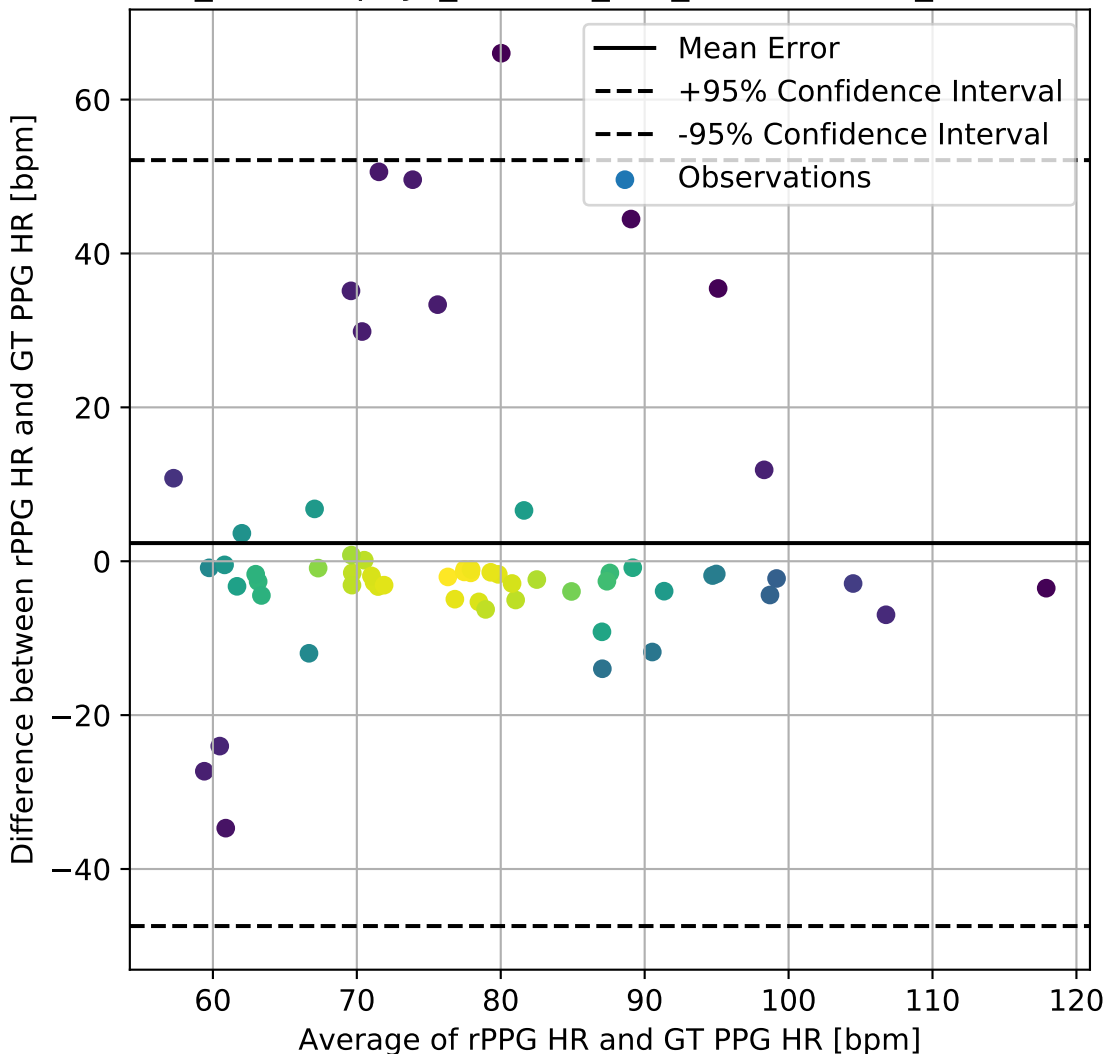
MA-UBFC_efficientphys_Custom_FFT_BlandAltman_DifferencePlot
