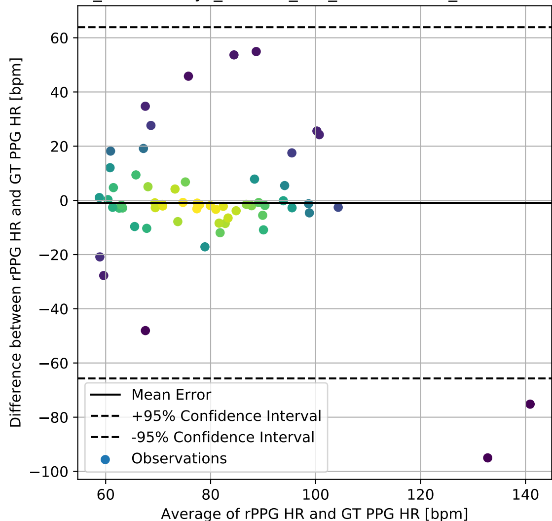
PURE EfficientPhys Custom FFT BlandAltman DifferencePlot
