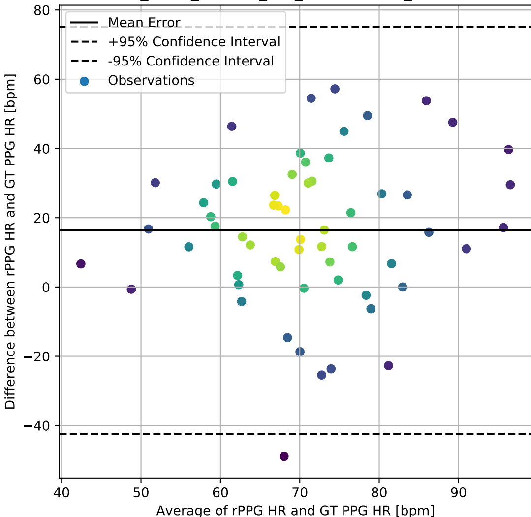
MA-UBFC_tscan_Custom_FFT_BlandAltman_DifferencePlot
