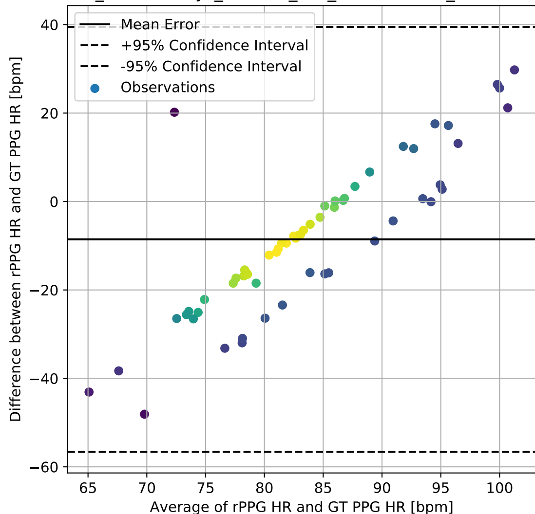
SCAMPS_EfficientPhys_Custom_FFT_BlandAltman_DifferencePlot
