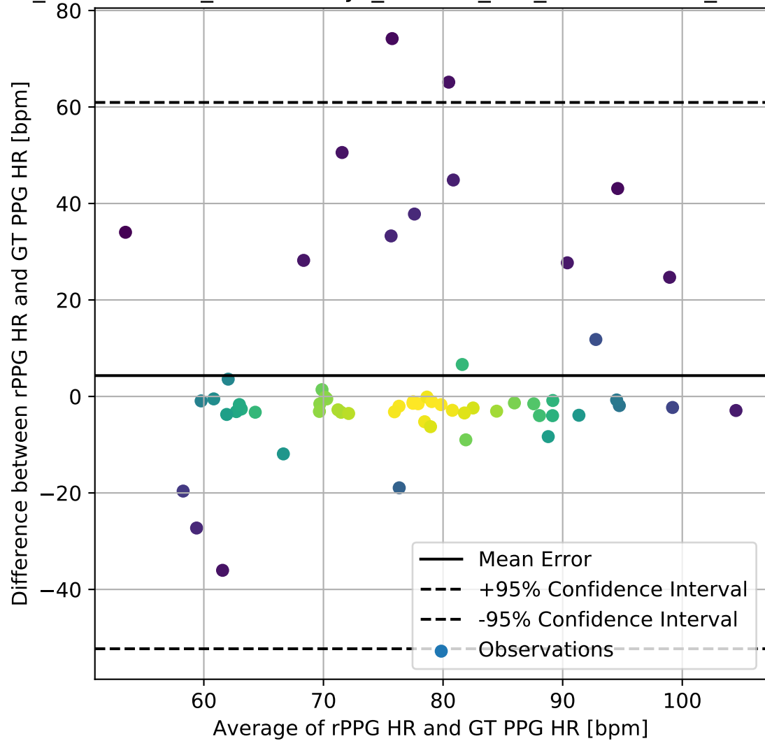
BP4D_PseudoLabel_EfficientPhys_Custom_FFT_BlandAltman_DifferencePlot
