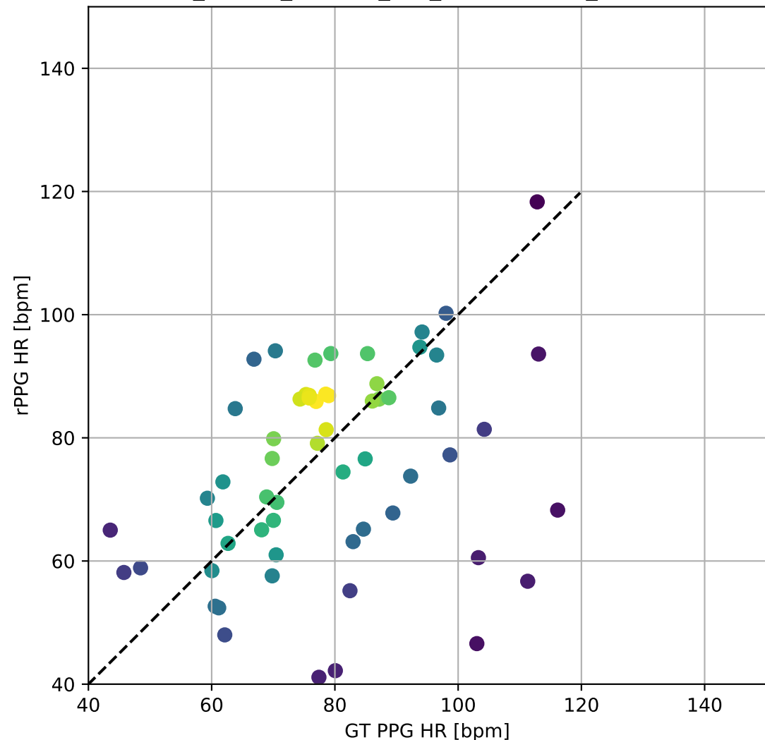
PURE_TSCAN_Custom_FFT_BlandAltman_ScatterPlot
