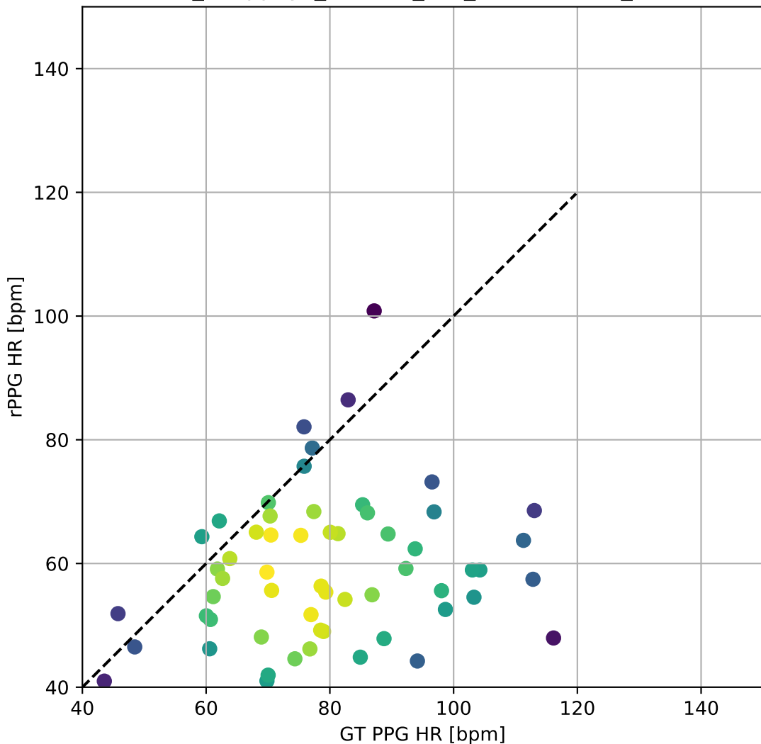
MA-UBFC_deepphys_Custom_FFT_BlandAltman_ScatterPlot
