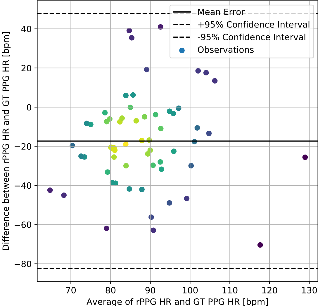
SCAMPS_PhysNet_DiffNormalized_Custom_FFT_BlandAltman_DifferencePlot
