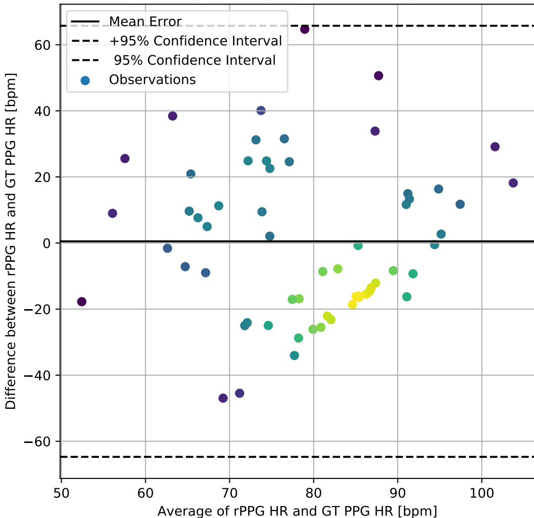
SCAMPS_TSCAN_Custom_FFT_BlandAltman_DifferencePlot
