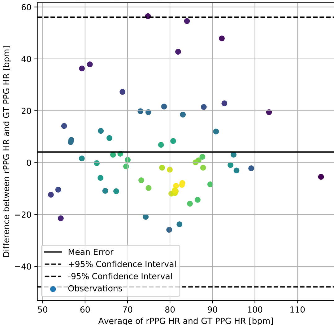
PURE_TSCAN_Custom_FFT_BlandAltman_DifferencePlot
