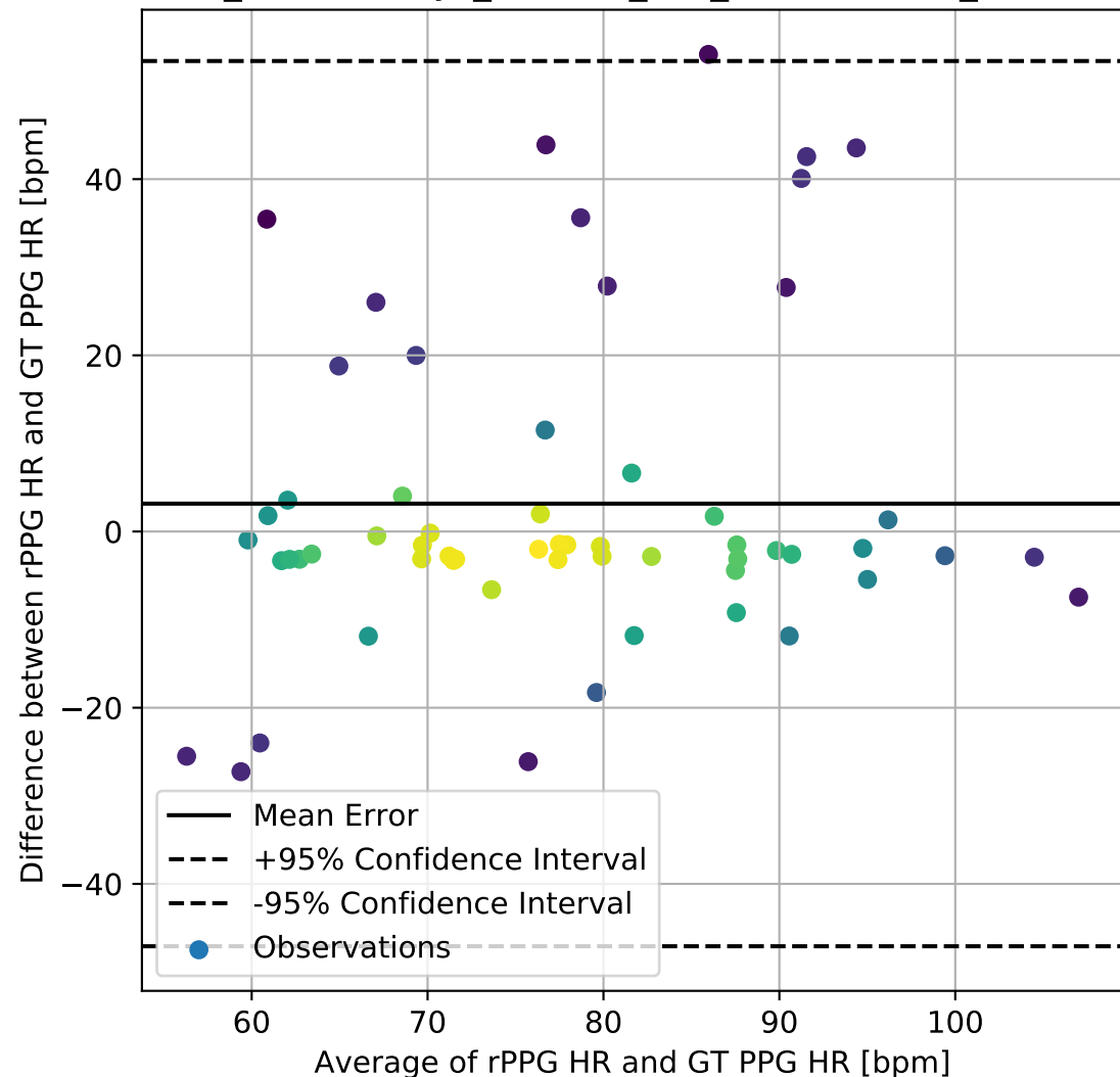
UBFC-rPPG_EfficientPhys_Custom_FFT_BlandAltman_DifferencePlot
