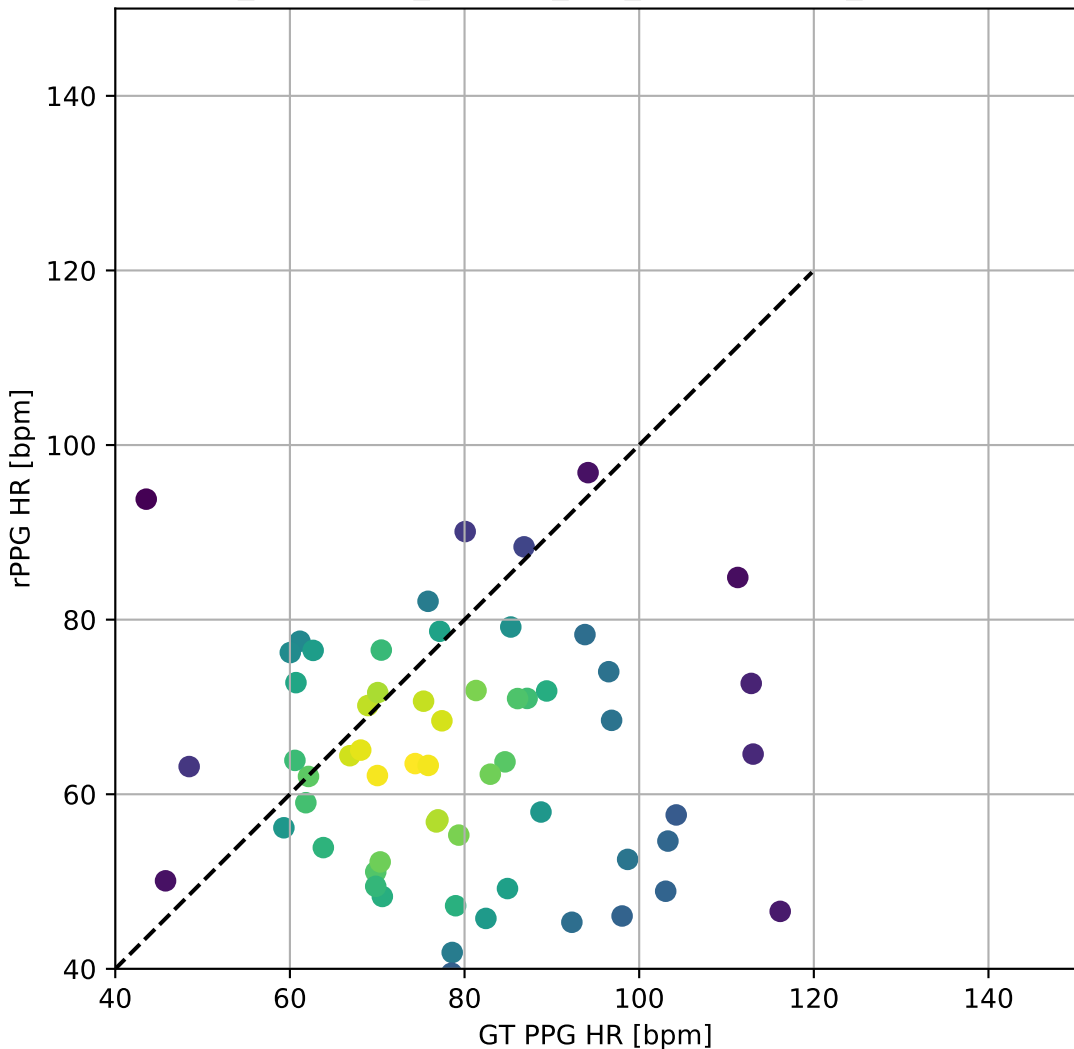
PURE_DeepPhys_Custom_FFT_BlandAltman_ScatterPlot
