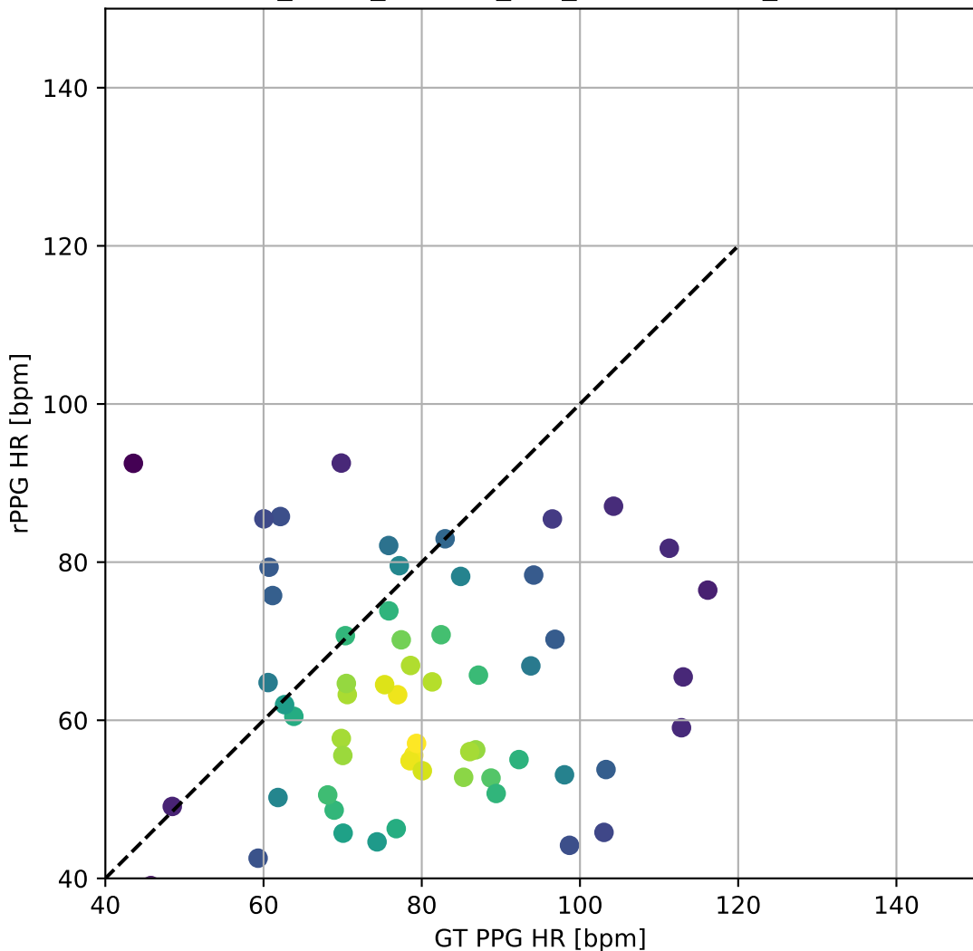
MA-UBFC_tscan_Custom_FFT_BlandAltman_ScatterPlot
