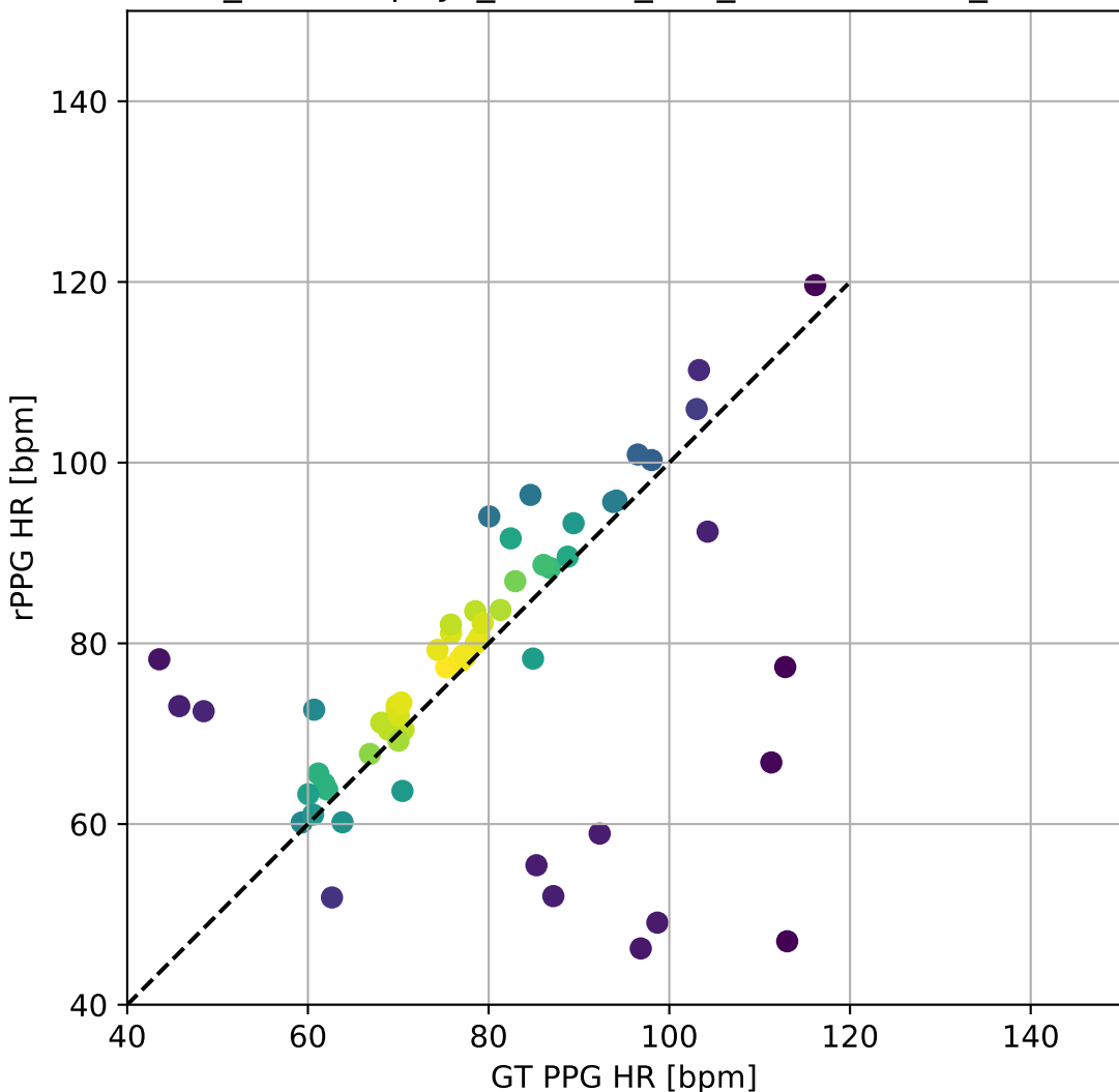
MA-UBFC_efficientphys_Custom_FFT_BlandAltman_ScatterPlot
