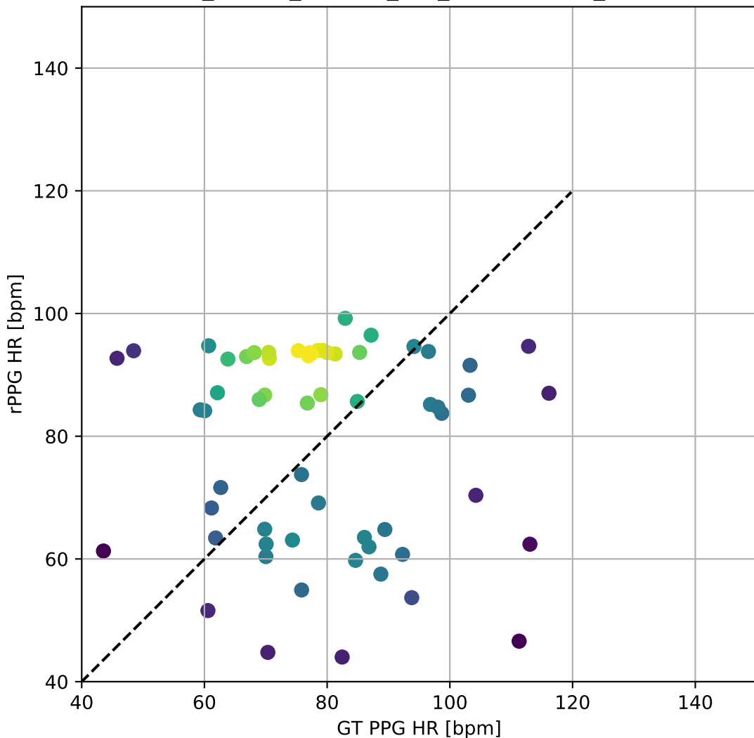
SCAMPS_TSCAN_Custom_FFT_BlandAltman_ScatterPlot
