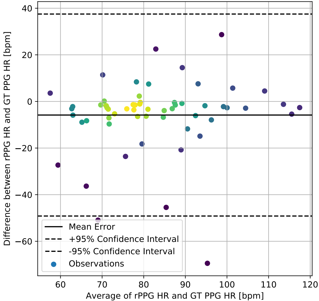
UBFC-rPPG_PhysNet_DiffNormalized_Custom_FFT_BlandAltman_DifferencePlot
