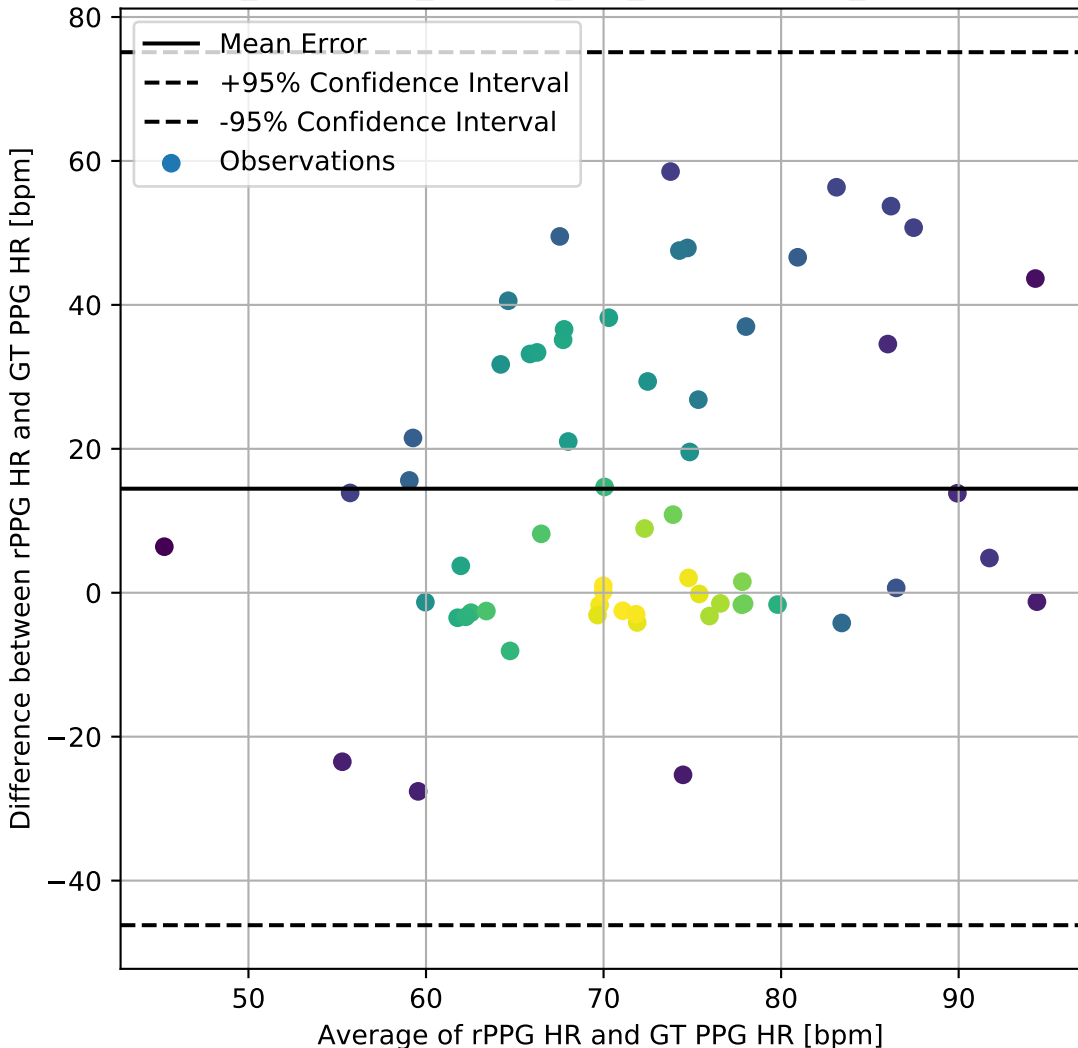
SCAMPS_DeepPhys_Custom_FFT_BlandAltman_DifferencePlot
