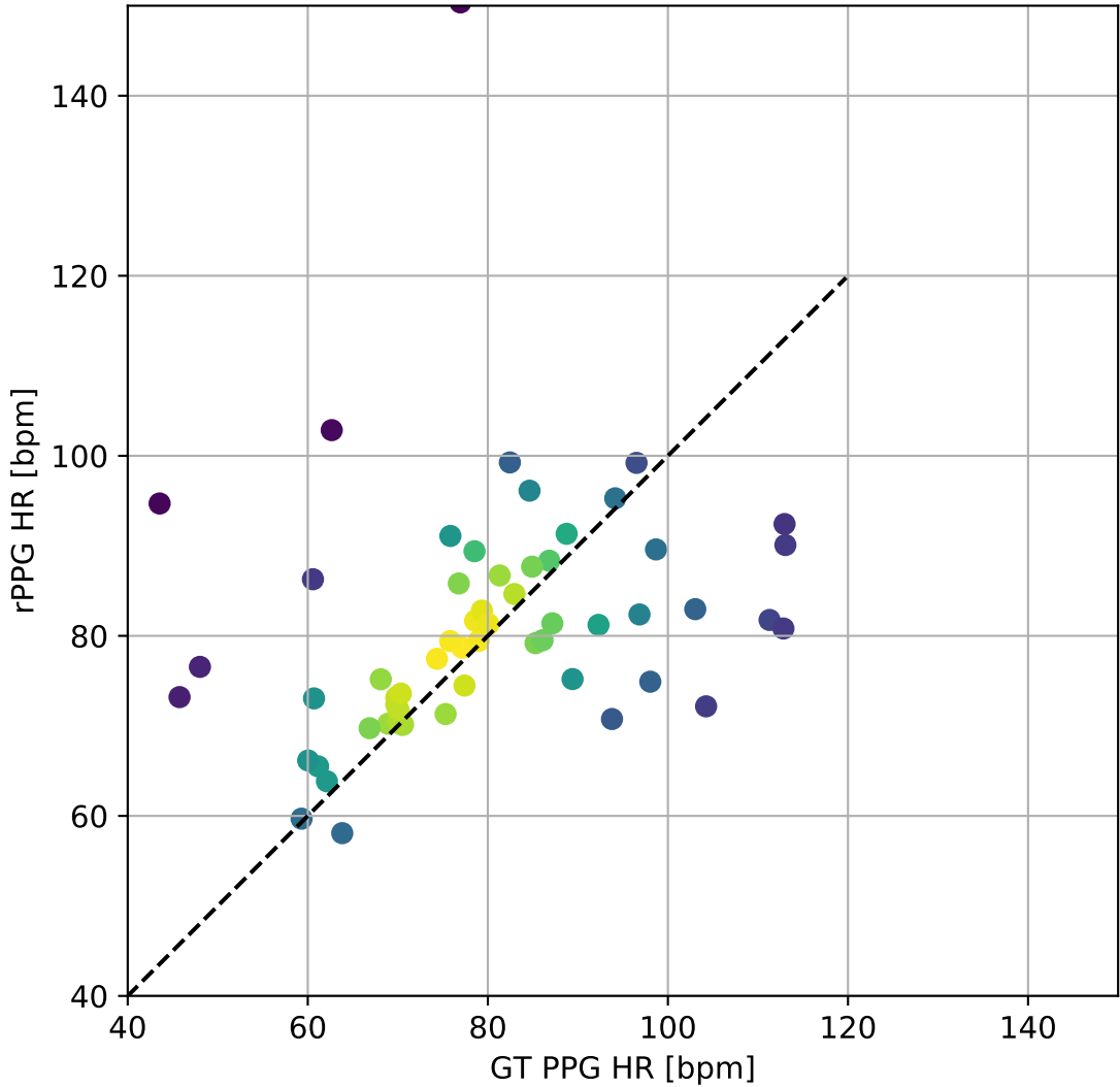
BP4D_PseudoLabel_PhysNet_DiffNormalized_Custom_FFT_BlandAltman_ScatterPlot
