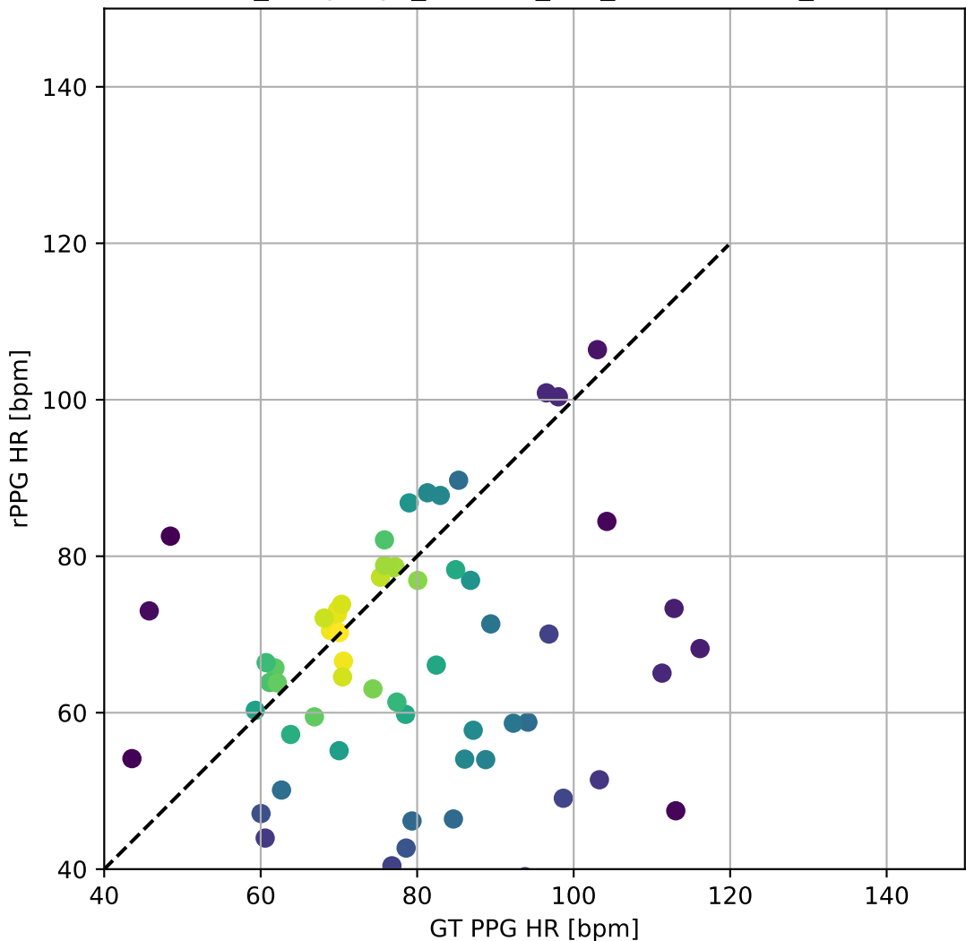
UBFC-rPPG_DeepPhys_Custom_FFT_BlandAltman_ScatterPlot
