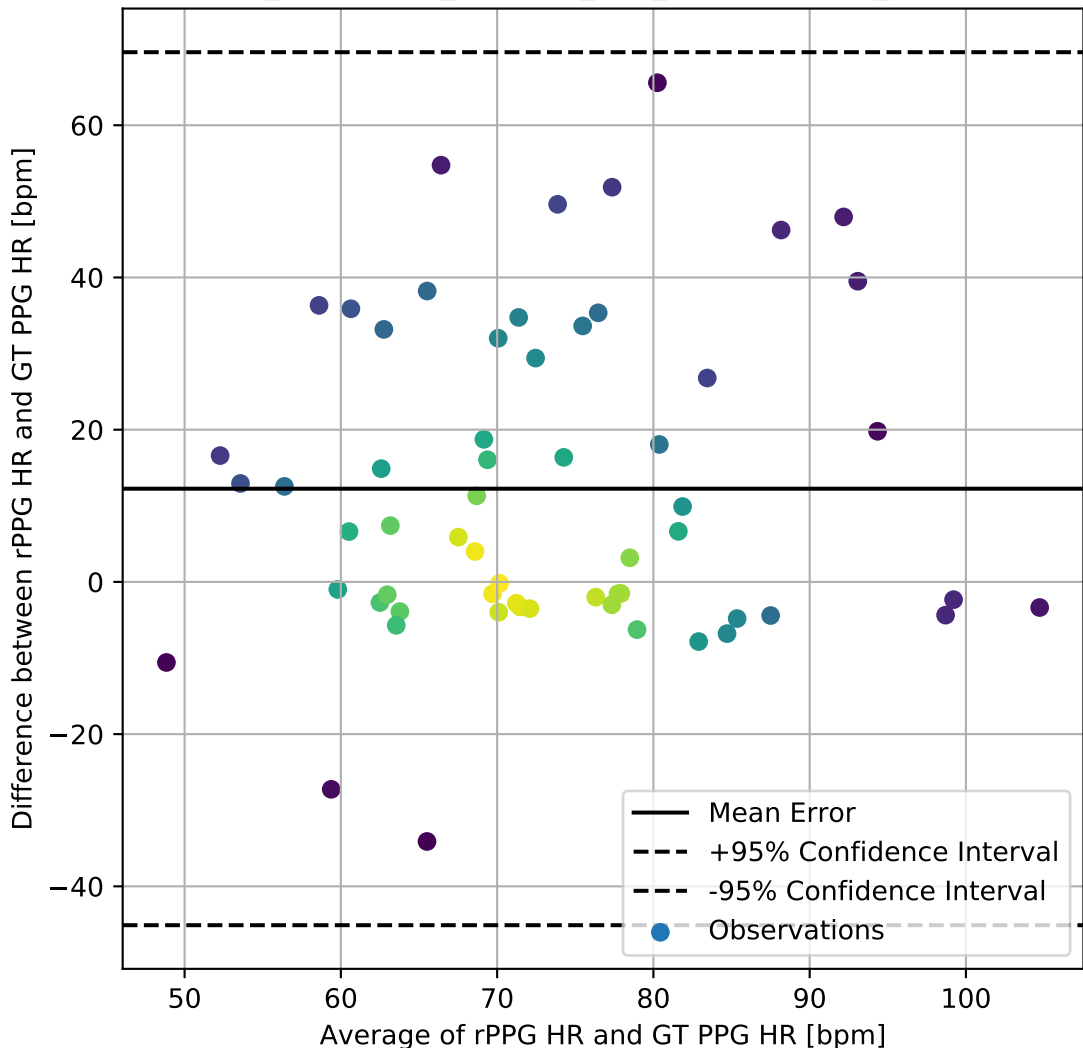
UBFC-rPPG_DeepPhys_Custom_FFT_BlandAltman_DifferencePlot
