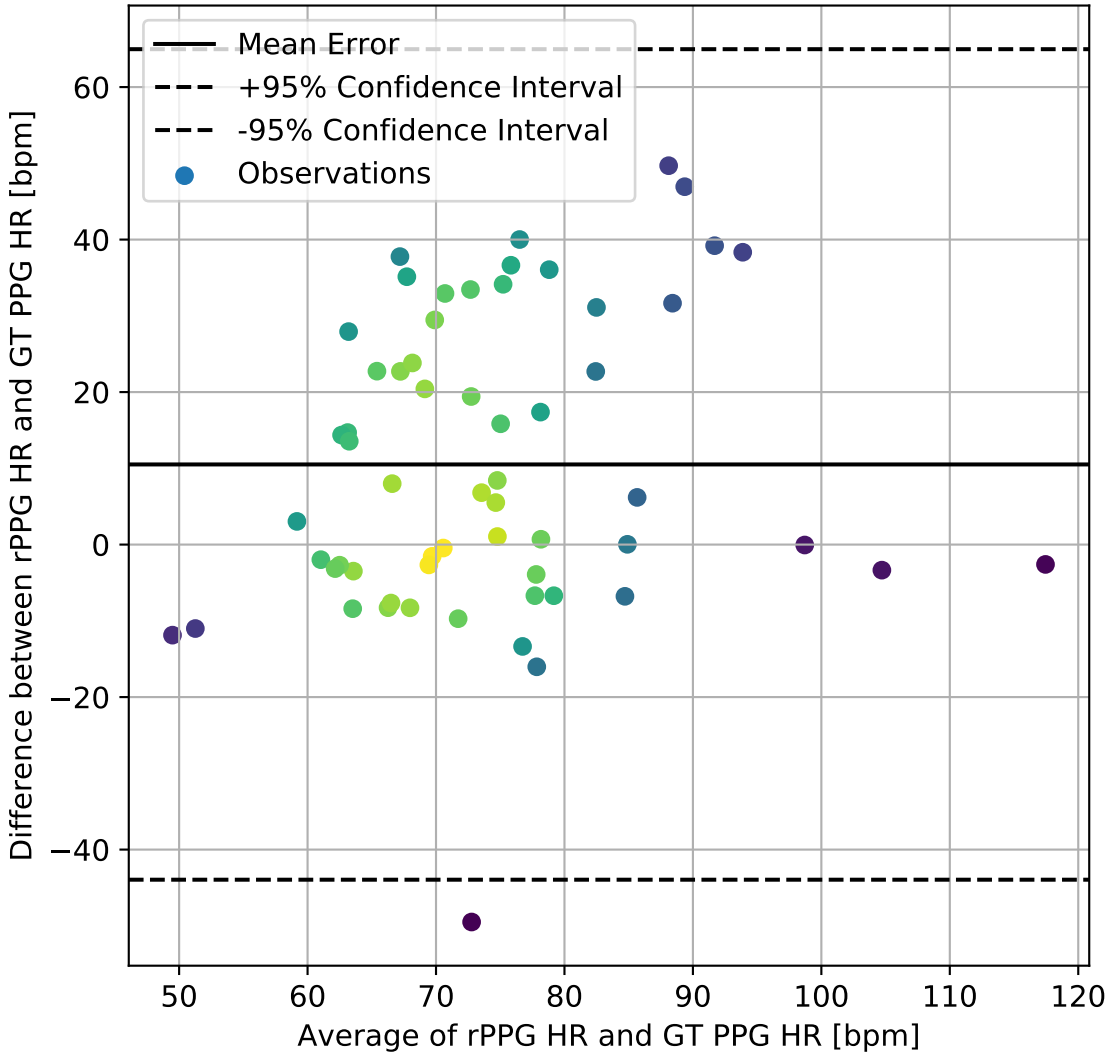
PURE_PhysNet_DiffNormalized_Custom_FFT_BlandAltman_DifferencePlot
