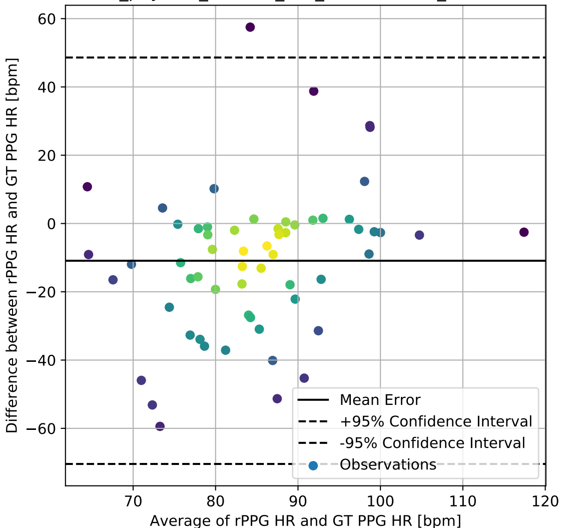
MA-UBFC_physnet_Custom_FFT_BlandAltman_DifferencePlot
