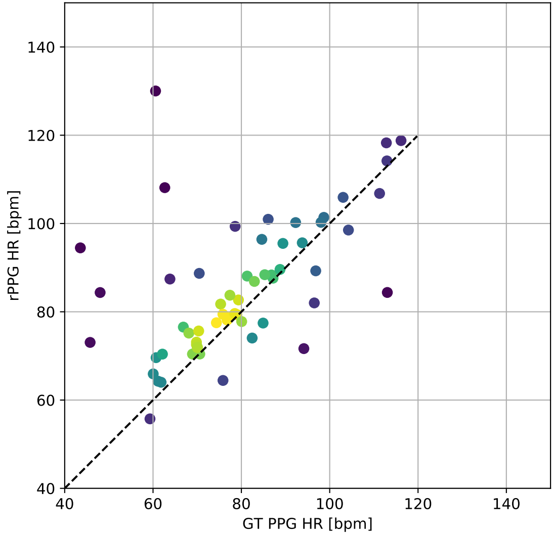
UBFC-rPPG_PhysNet_DiffNormalized_Custom_FFT_BlandAltman_ScatterPlot
