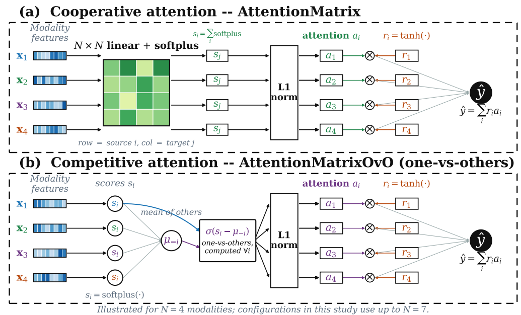
Figure 3. Architecture of the two attention mechanisms. Both variants compute a per-modality risk score r_i = \tanh(\mathbf{W}_{r,i}^T \mathbf{x}_i) (Equation 1) and produce the fused prediction \hat{y} = \sum_i r_i a_i (Equation 6); they differ only in how the attention weights a_i are obtained. (A) Cooperative attention ( AttentionMatrix ): an N \times N grid of linear layers with softplus activation produces pairwise scores that are column-summed into s_j (Equation 2) and L1-normalised so that the modalities share a fixed attention budget (Equation 3). (B) Competitive one-vs-others attention ( AttentionMatrixOvO ): each modality produces a single score s_i that is compared against the mean score of the remaining modalities \mu_{-i} through a sigmoid, \sigma(s_i - \mu_{-i}) (Equations 4–5), yielding an independent competitive weight before L1 normalisation. Heatmap bars denote modality feature vectors; the diagram is drawn for N = 4 modalities for clarity.
