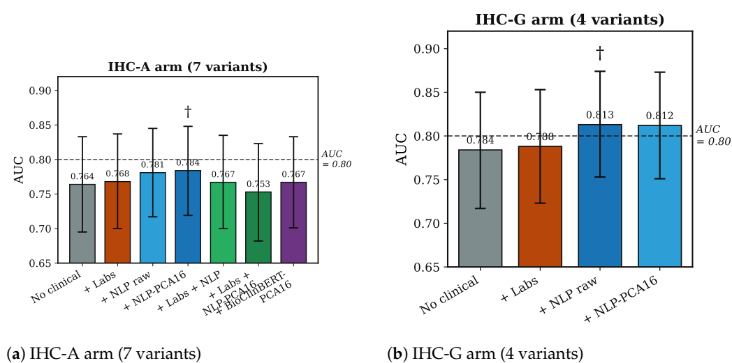
Figure 4. AUC comparison across clinical encoding strategies for (A) the IHC-A arm and (B) the IHC-G arm. Bars show pooled out-of-fold AUC from 10-fold cross-validation ( n = 247 ); error bars denote DeLong 95% confidence intervals. The dashed horizontal line at AUC = 0.80 indicates the conventional threshold for clinically useful discrimination. † Best-performing model overall (DyAM Rad+IHC-G+Gen+PDL1+NLP raw, AUC = 0.813 ).
