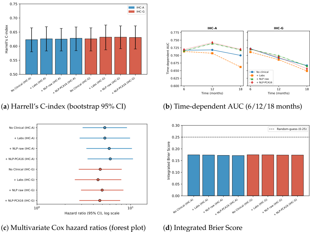
Figure 6. Survival analysis summary across clinical encoding strategies. (A) Harrell’s C-index with bootstrap 95% confidence intervals for IHC-A and IHC-G arms; differences between encoding strategies were not statistically significant (paired Wilcoxon p > 0.05 ). (B) Time-dependent AUC at 6, 12, and 18 months; NLP-encoded models show the largest advantage at 12–18 months. (C) Forest plot of multivariate Cox proportional hazards ratios for the fused risk score, adjusted for age, ECOG performance status, albumin, derived neutrophil-to-lymphocyte ratio, and liver metastases (all p < 0.001 ). (D) Integrated Brier Score (IBS) for each model; all values fall well below the 0.25 random-guess threshold (range 0.172–0.175), indicating good calibration across all encoding strategies.
