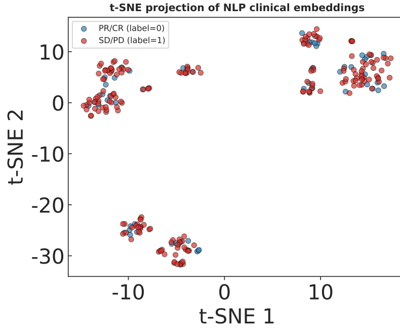
Figure S2: Two-dimensional t-SNE projection of the 384-dimensional NLP clinical embeddings for all n = 247 discovery-cohort patients, coloured by binary outcome (blue: PR/CR, label = 0; red: SD/PD, label = 1). The substantial overlap between classes is consistent with the embeddings encoding general clinical/prognostic similarity rather than a strong linear separation of binary treatment response, in agreement with the survival-dominant signal described in the Survival Analysis section of the main text.
