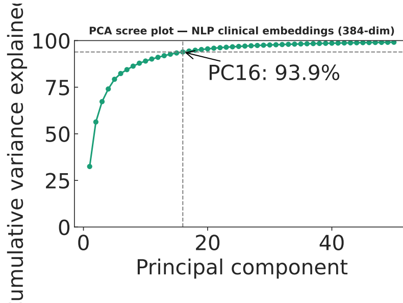
Figure S1: PCA scree plot for the 384-dimensional NLP sentence embeddings. The x-axis shows the principal component number (1–50) and the y-axis shows cumulative variance explained (%). The first 16 components (vertical dashed line, used as “NLP-PCA16”) jointly explain \approx 94\% of total variance.
