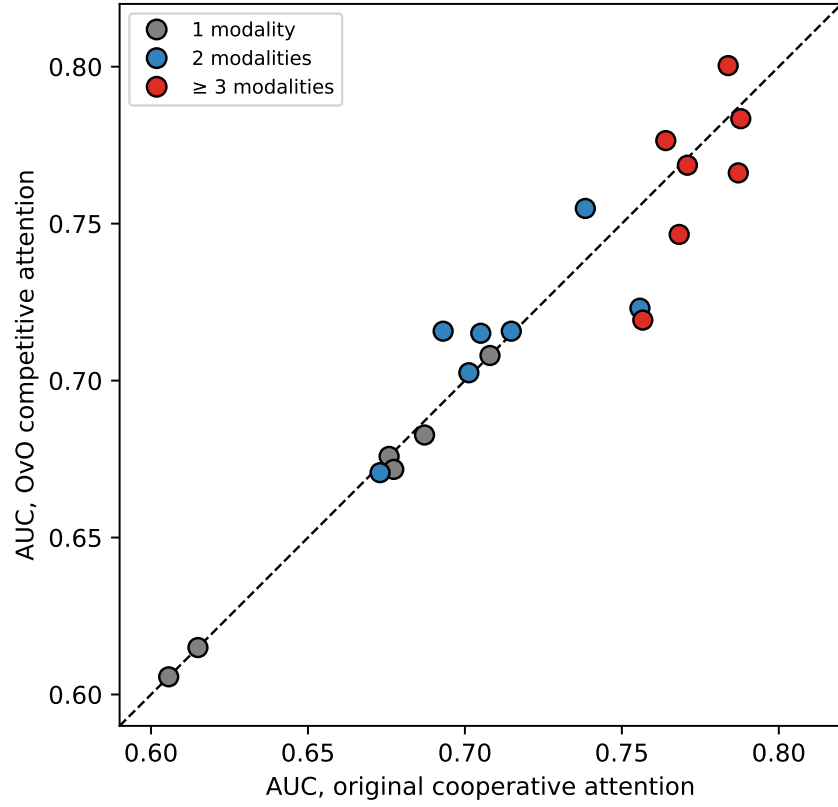
Figure S4: Scatter plot comparing AUC under the original cooperative attention (x-axis) versus OvO competitive attention (y-axis) across all 20 tested modality configurations. The diagonal line indicates equal performance. Points are coloured by the number of fused modalities (grey: 1 modality, where OvO reduces to the original formulation; blue: 2 modalities; red: \geq 3 modalities). Points above the diagonal indicate configurations where OvO attention improved AUC.
