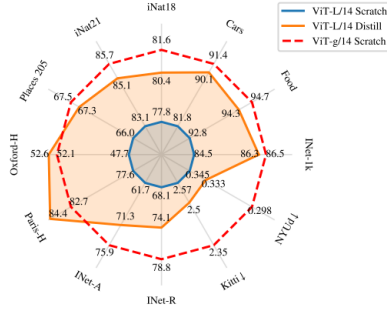
(a) Comparison on individual metrics
