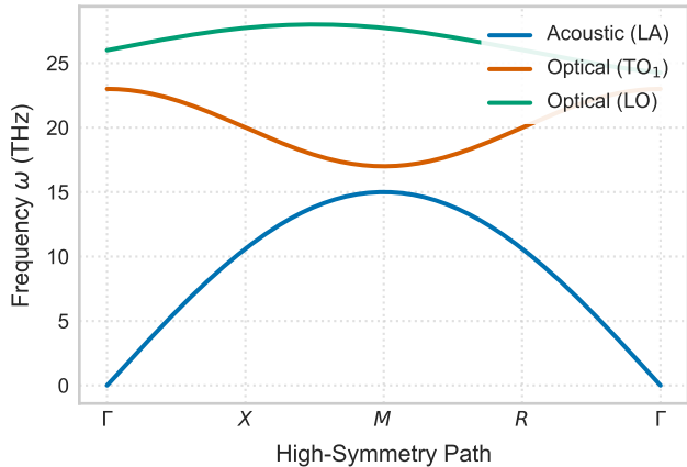
\textbf{a} Phonon Dispersion
