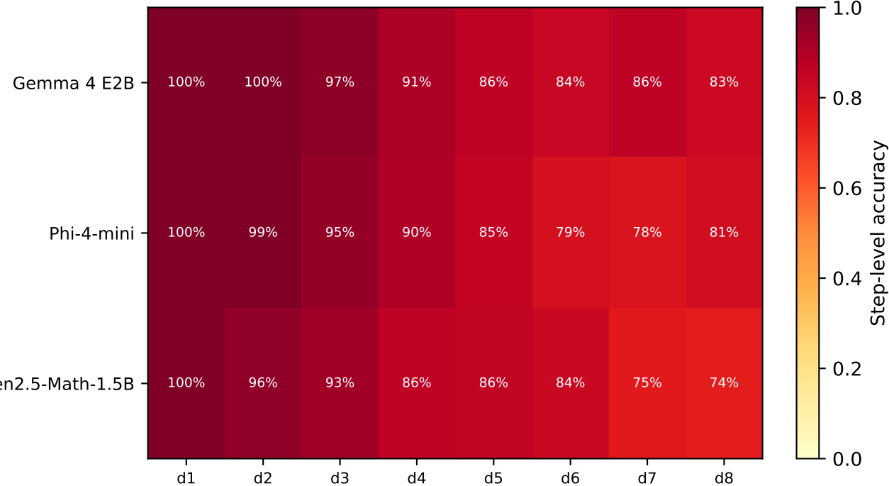
Step-Level Accuracy — CoT
