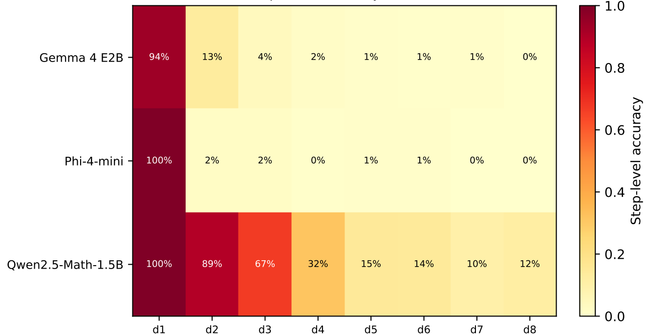
Step-Level Accuracy — Direct
