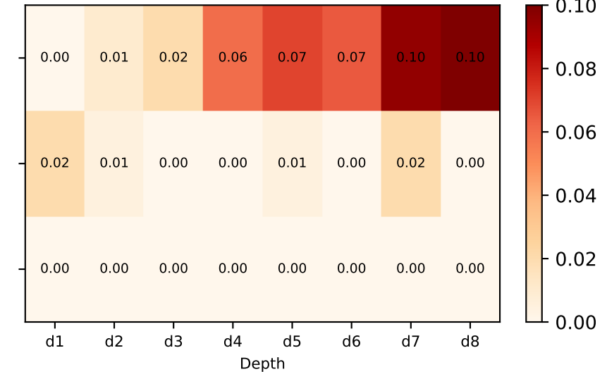
Qwen2.5-Math-1.5B
