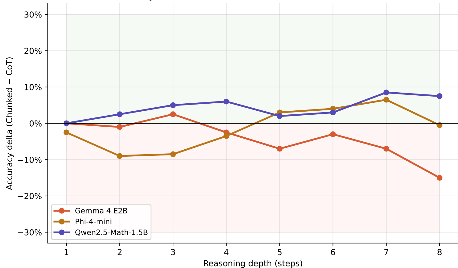
Accuracy Gain / Loss of Chunked Method vs CoT Baseline
