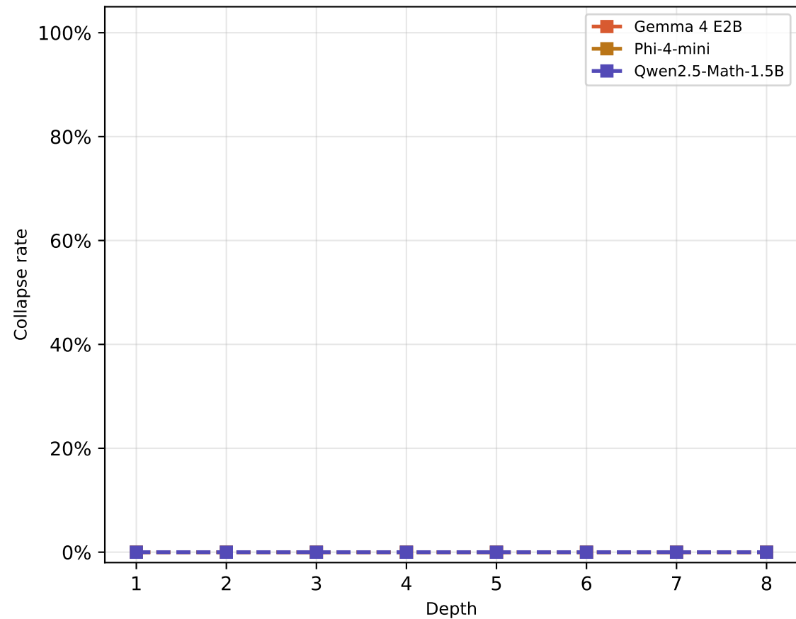
Output Collapse — Direct
