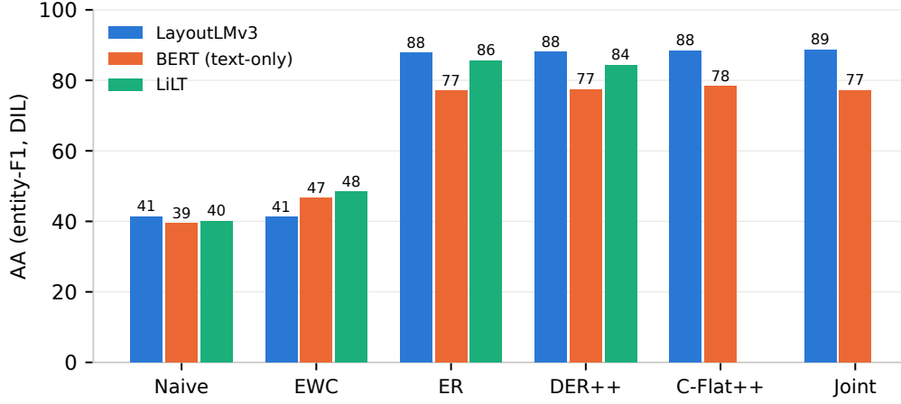
Figure 6.13: The replay-dominant ordering on DIL across backbones (mean over three seeds, from the aggregated run table). The three-tier structure—replay near the joint oracle, regularisation barely above the naive floor—reproduces on the text-only BERT backbone at a uniformly lower level and on LiLT where cells exist; C-Flat++ and Joint are not yet run on LiLT.
