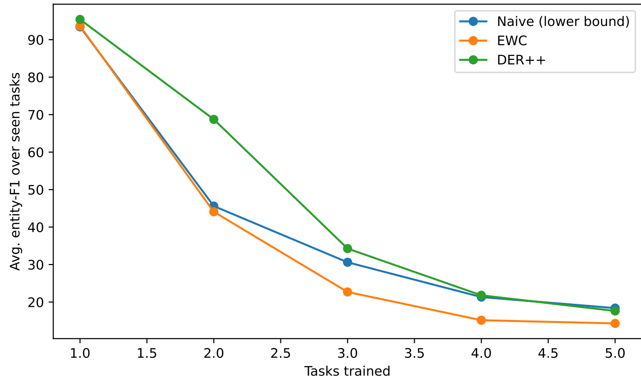
Forgetting curves (CIL-CORD)
