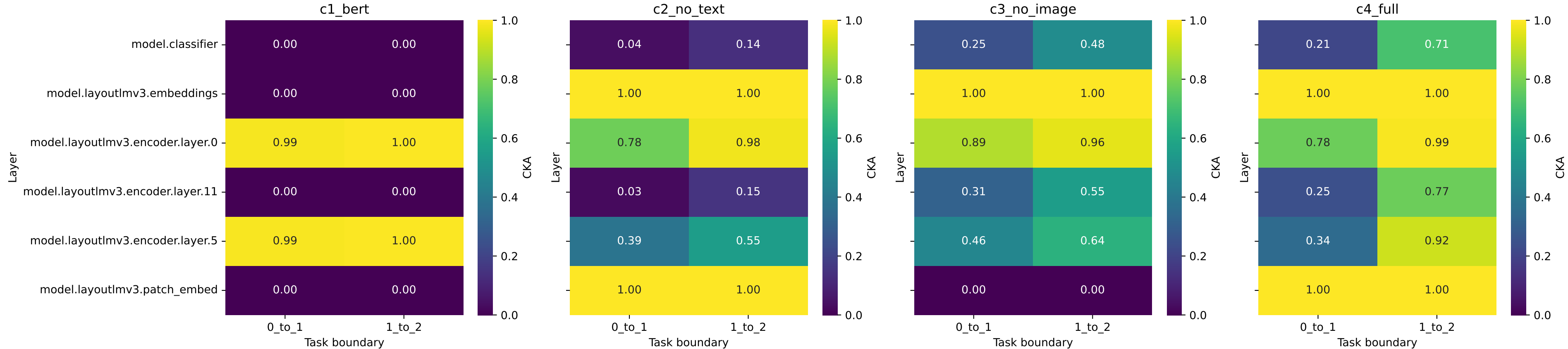
Per-layer CKA between consecutive task checkpoints
