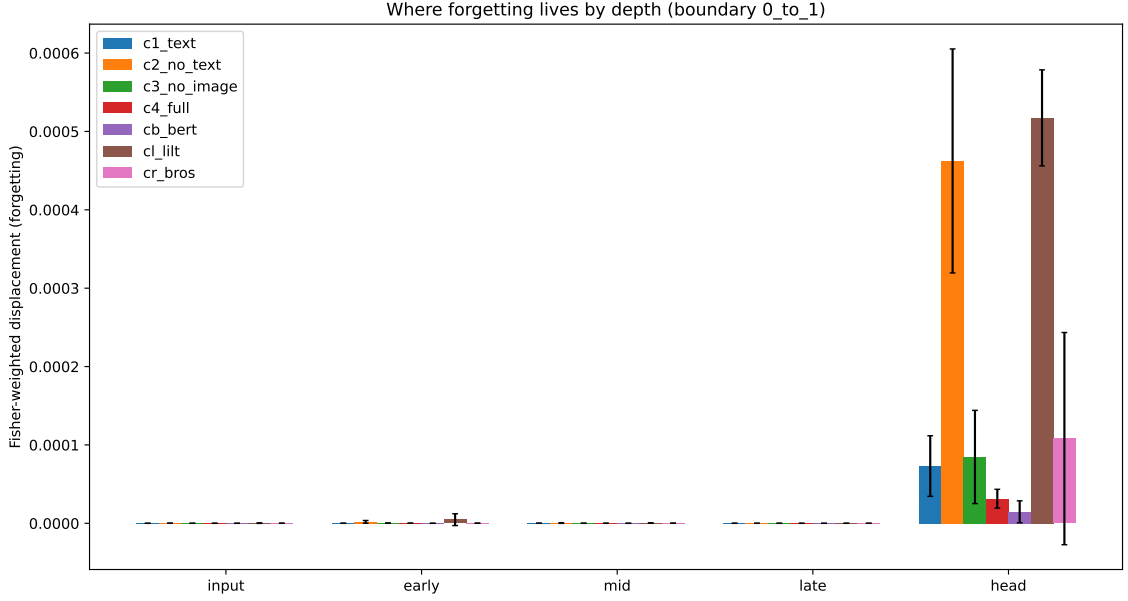
Figure 6.1: Per-component forgetting localiser: old-task-Fisher-weighted displacement D_g by depth bucket, grouped by backbone condition—large where parameters important to the previous task were overwritten. Across every condition (the four LayoutLMv3 modality masks, the BERT text-only baseline, and the LiLT and BROS secondary backbones), the classifier head’s weighted displacement is one-to-four orders of magnitude larger than any encoder layer’s: forgetting concentrates at the classifier head and late encoder layers while the input encoders barely move, and the profile is statistically the same across all four architectures (§6.1.3).
