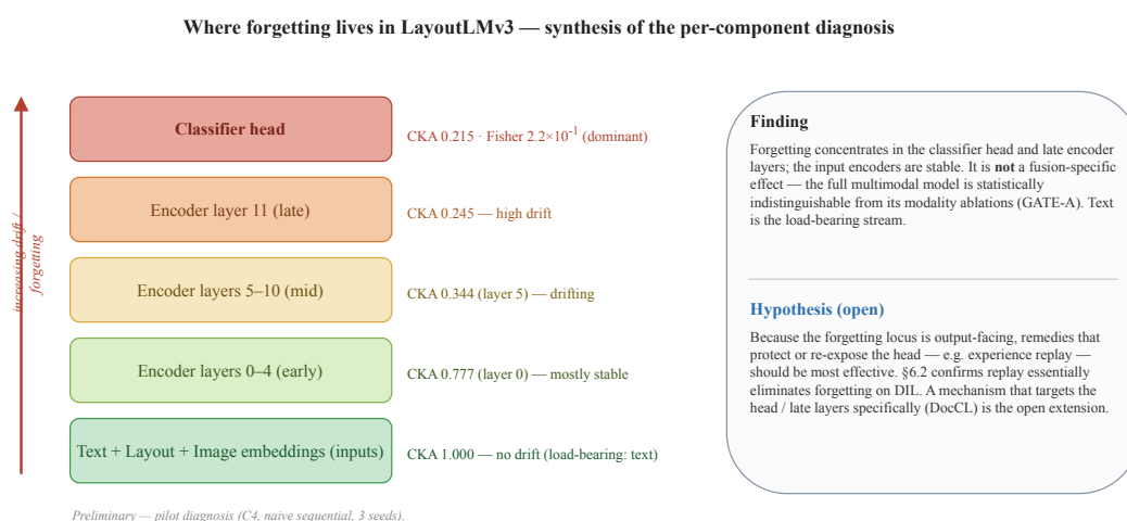
Figure 6.4: Synthesis of the per-component diagnosis on the LayoutLMv3 stack: drift and parameter importance increase with depth, peaking at the classifier head, while the input encoders are stable. The panel states the data-supported finding and the diagnosis-grounded (open) hypothesis. Pilot result.
