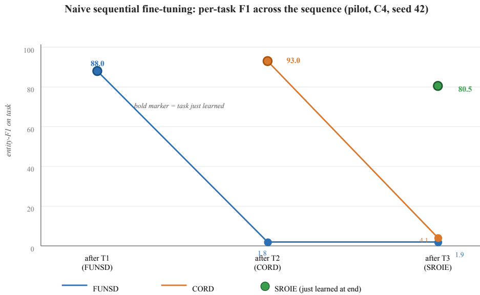
Figure 6.10: Per-task entity-F1 as the naive sequential pilot progresses (C4, seed 42). Each task is learned to a strong F1 when it is the current task (bold markers: 88.0 / 93.0 / 80.5) and then collapses to ~2–4 F1 once the next task is trained — the rows of Table 6.1 read left to right. Pilot result (seed 42).
