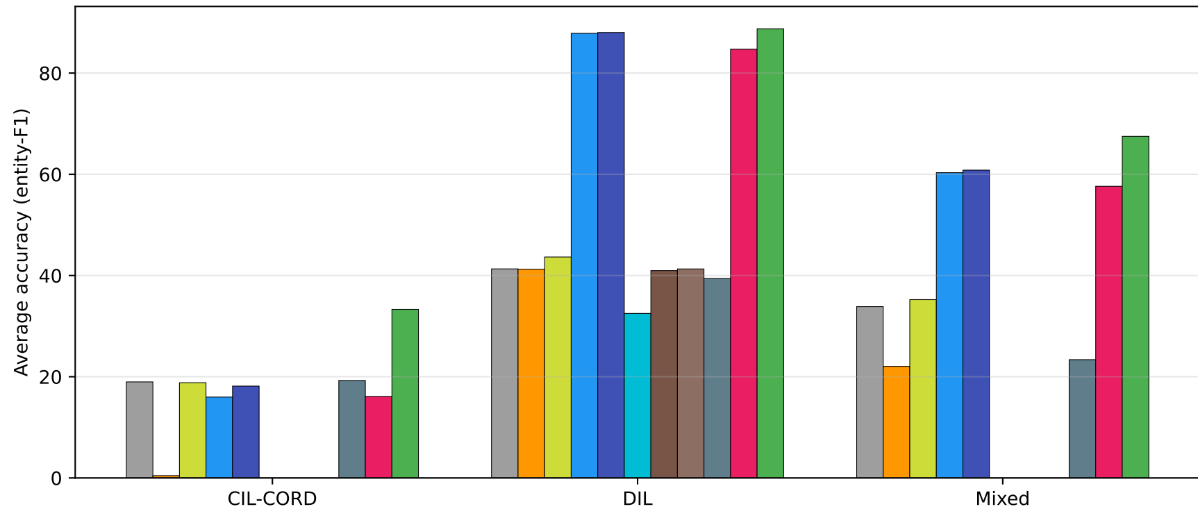
Average accuracy by method and scenario Naive W Lora ER Joint EWC ER CODA-Prompt CL-LoRA DocCL
