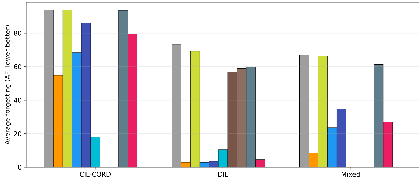
Average forgetting by method and scenario Naive Low ER CODA-Prompt CL-LoRA DocCL Joint EWC
