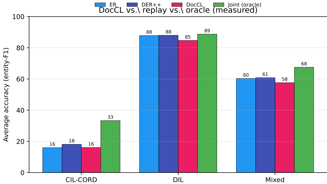
Figure 6.8: Focused comparison of the proposed DocCL against the strongest baselines (ER, DER++) and the joint oracle, average entity-F1 per scenario (all measured). DocCL closes most of the domain-incremental forgetting gap (within ~4 points of the oracle) but does not reach it; the replay methods match the oracle and remain ~3 points ahead of DocCL on DIL and clearly ahead on Mixed; on the hard CIL-CORD scenario no method makes real progress.
