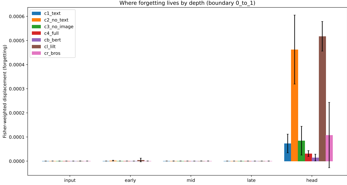
Figure 6.1: Per-component forgetting localiser: old-task-Fisher-weighted displacement D_g by depth bucket, grouped by backbone condition—large where parameters important to the previous task were overwritten. Across every condition (the four LayoutLMv3 modality masks, the BERT text-only baseline, and the LiLT and BROS secondary backbones), the classifier head’s weighted displacement is one-to-four orders of magnitude larger than any encoder layer’s: forgetting concentrates at the classifier head and late encoder layers while the input encoders barely move, and the profile is statistically the same across all four architectures (§6.1.3).
