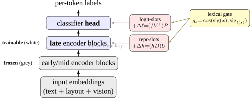
Figure 3.5: LexSlot places small additive slot adapters at the diagnosed forgetting locus over a partially-frozen backbone. The lower 2/3 encoder (grey) is frozen so stable pre-trained features flow into the slots without drifting; the late blocks and the classifier head (white) stay trainable and carry the slots—the trainable set is exactly the slot-bearing set, and the dashed line marks the freeze boundary. Logit-slots add a per-token bias \Delta \ell at the head; repr-slots add a low-rank shift \Delta h in the late blocks. Up-projections are zero-initialised, so an untrained slot is an exact no-op. The inference lexical gate (yellow) scales each slot’s activation at forward time by the cosine between the document’s signature and the slot’s owner-task signature, routing the right memory to the right document at prediction time (active in both training and inference; §3.4.3).
