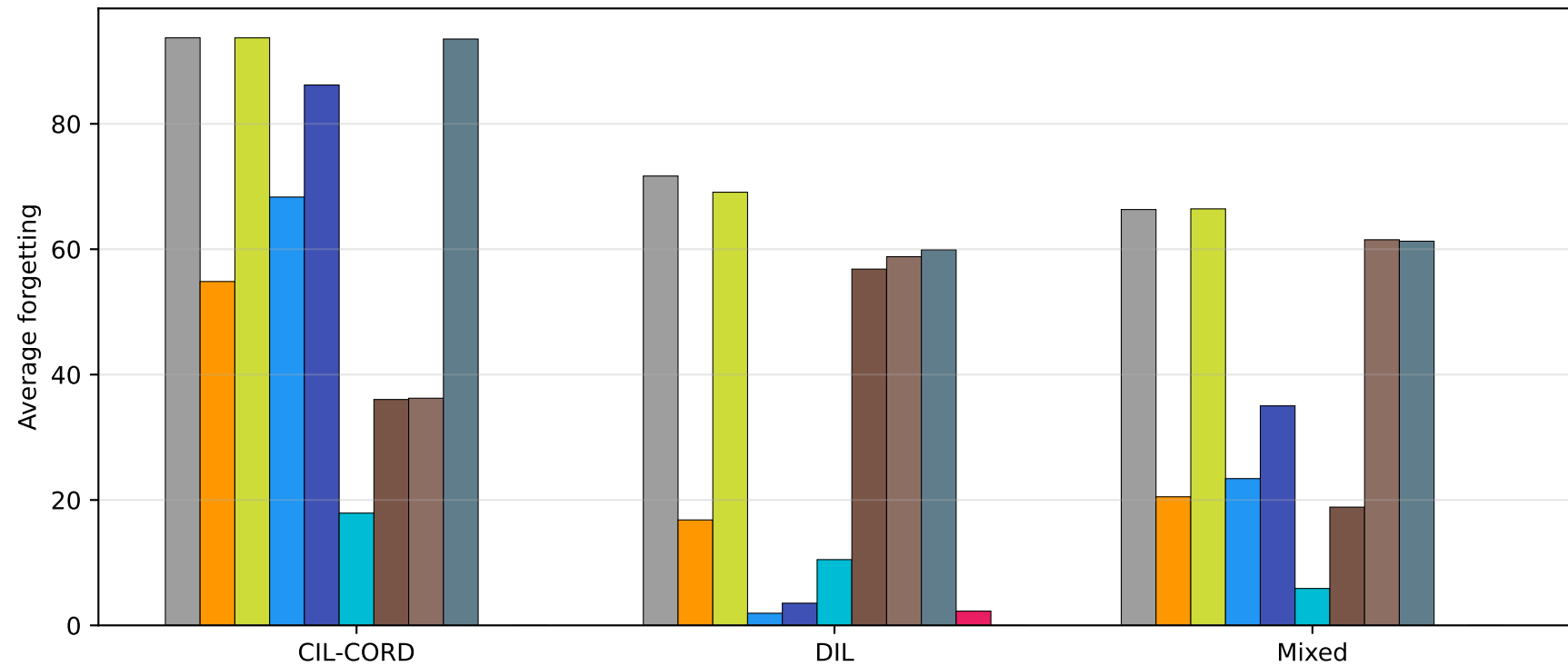
Average forgetting by method and scenario
