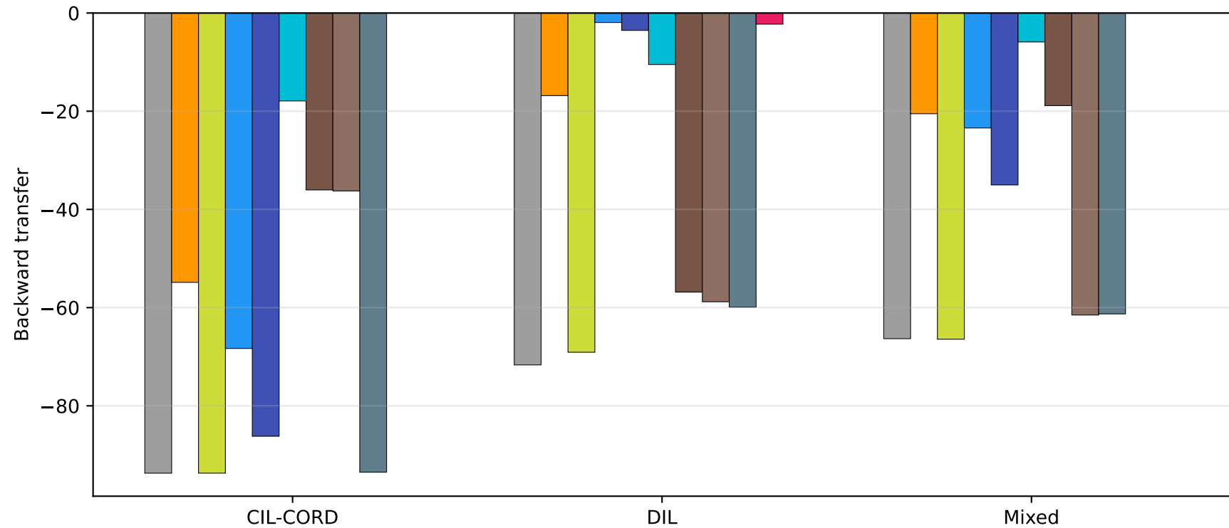
Backward transfer by method and scenario
