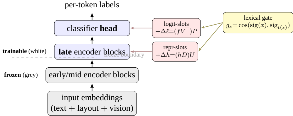
Figure 3.5: LexSlot places small additive slot adapters at the diagnosed forgetting site over a partially-frozen backbone. The lower 2/3 encoder (grey) is frozen so stable pretrained features flow into the slots without drifting; the late blocks and the classifier head (white) stay trainable and carry the slots, the trainable set is exactly the slot-bearing set, and the dashed line marks the freeze boundary. Logit-slots add a per-token bias \Delta\ell at the head; repr-slots add a low-rank shift \Delta h in the late blocks. Up-projections are zero-initialised, so an untrained slot is an exact no-op. The inference lexical gate (yellow) scales each slot’s activation at forward time by the cosine between the document’s signature and the slot’s owner-task signature, routing the right memory to the right document at prediction time (active in both training and inference; §3.4.3).
