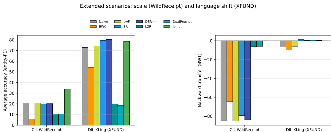
Figure 6.14: Average accuracy on the two extended scenarios. Left : WildReceipt class-incremental learning (scale axis; classical methods and joint oracle shown), where forgetting is severe and even replay stays near the naive lower bound, far below the oracle. Right : XFUND cross-lingual DIL (pure language shift, fixed label space), where forgetting is near zero for every method: naive already reaches 72.9 AA and replay edges past the oracle, because the fixed output space never forces the head to relearn its distribution. The contrast corroborates the output-side / head-site forgetting thesis.
