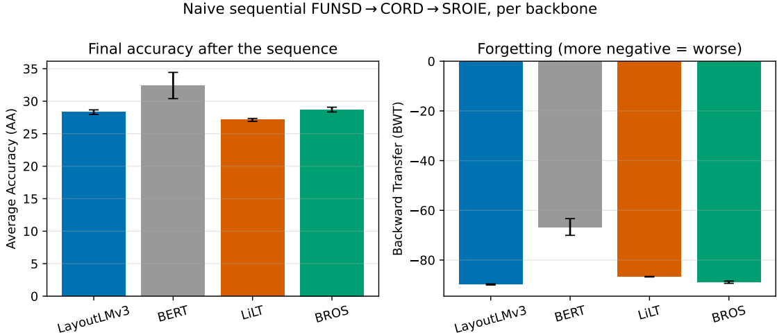
Figure 6.5: Continual-learning metrics by backbone under naive sequential FUNSD \rightarrow CORD \rightarrow SROIE (mean \pm std over three seeds). Left: final average accuracy. Right: backward transfer (more negative = more forgetting). The three multimodal/layout backbones (LayoutLMv3, LiLT, BROS) forget heavily and comparably; the text-only BERT baseline forgets somewhat less. Differences between backbones are within the regime expected at this seed count and are not over-interpreted.
