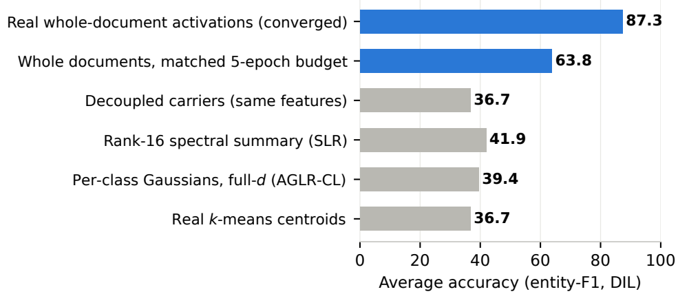
Figure 6.15: The latent-replay elimination ladder at a fixed frozen boundary (layer k=8 , DIL). Only whole-document replay (blue) retains accuracy; every summarised representation, including real k -means centroids, collapses to the naive level, and the matched-budget single-variable control (whole documents 63.8 vs. the same features on decoupled carriers 36.7) isolates whole-document (feature, position, label) binding as the necessary ingredient. Single-seed diagnostic runs (seed 42).
