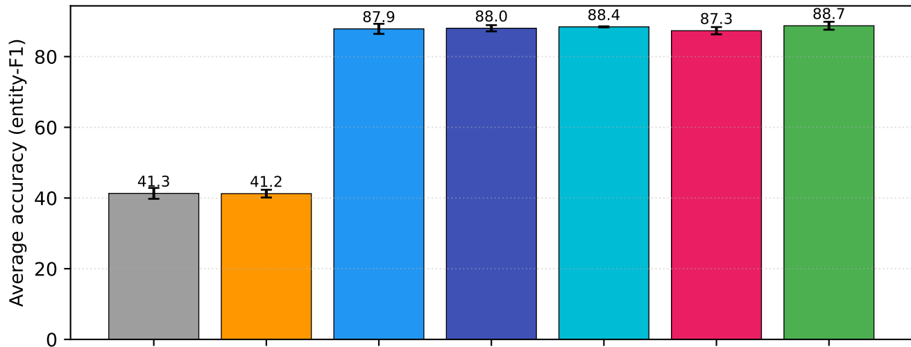
Domain-incremental (DIL): LexSlot vs baselines (mean over seeds, \pm std)
