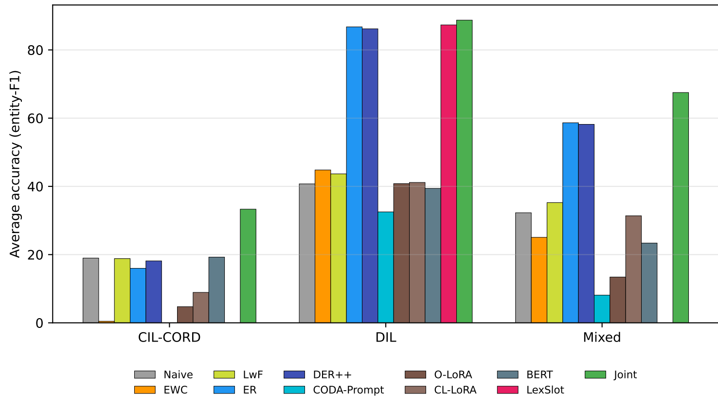
Average accuracy by method and scenario
